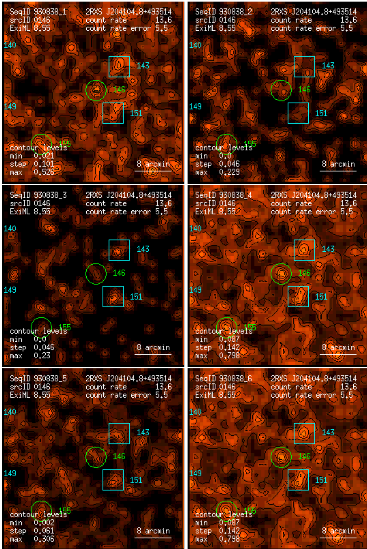
Figure 146: RASS 930838: detection 0146: band rate images, Gaussian filter: (1) PSPC channels 11 – 41, (2) 52 – 90, (3) 91 – 201, (4) 11 – 235, (5) 52 – 201, (6) 11 – 201. Broad band rates in counts/ks. Band rate contour levels in counts/ks/arcmin 2 .
