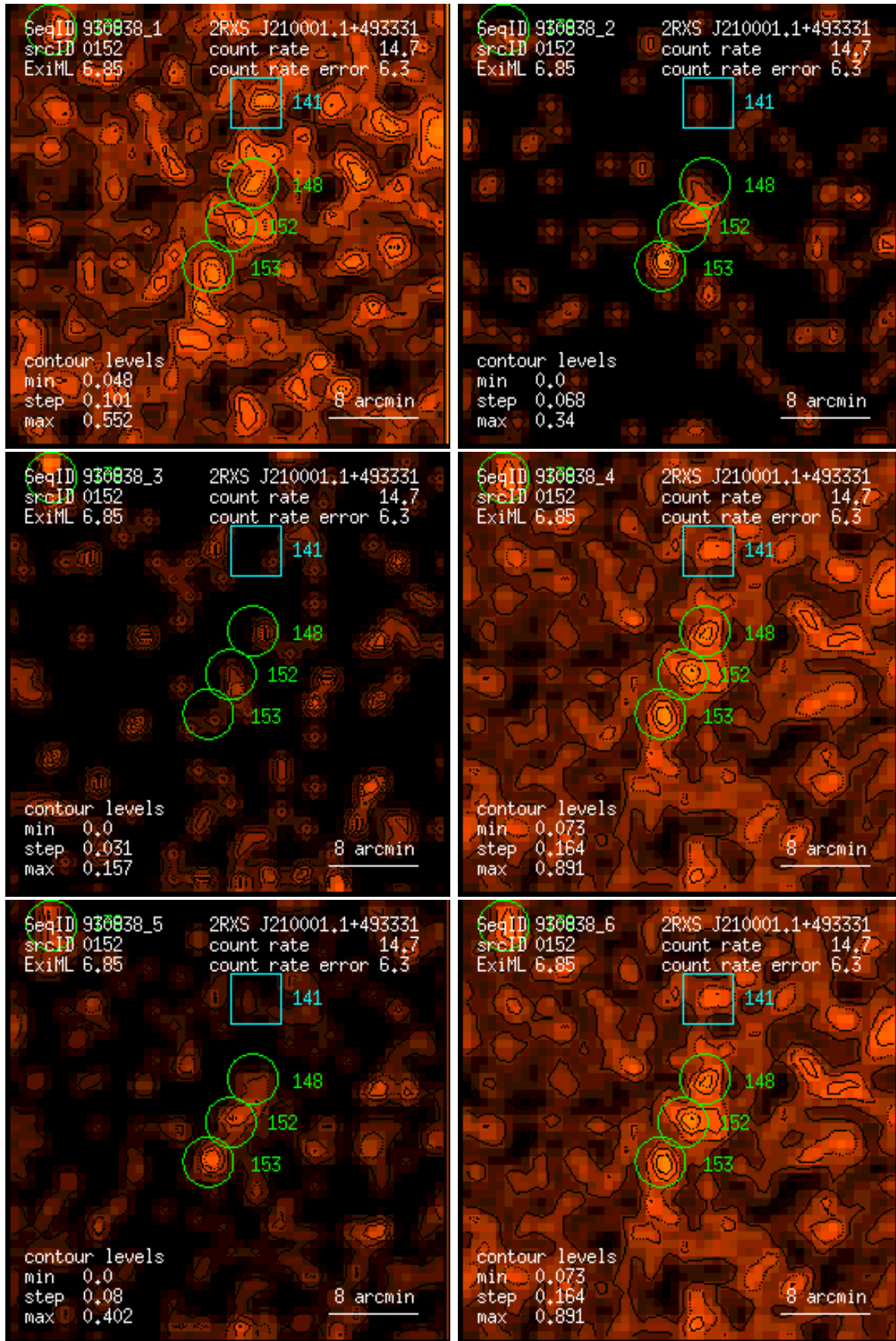
Figure 152: RASS 930838: detection 0152: band rate images, Gaussian filter: (1) PSPC channels 11 – 41, (2) 52 – 90, (3) 91 – 201, (4) 11 – 235, (5) 52 – 201, (6) 11 – 201. Broad band rates in counts/ks. Band rate contour levels in counts/ks/arcmin 2 .
