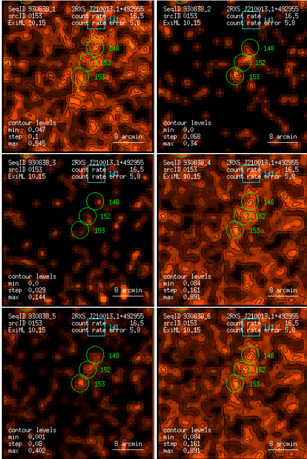
Figure 153: RASS 930838: detection 0153: band rate images, Gaussian filter: (1) PSPC channels 11 – 41, (2) 52 – 90, (3) 91 – 201, (4) 11 – 235, (5) 52 – 201, (6) 11 – 201. Broad band rates in counts/ks. Band rate contour levels in counts/ks/arcmin 2 .
