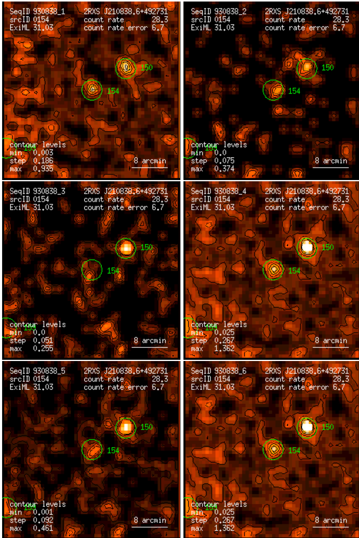
Figure 154: RASS 930838: detection 0154: band rate images, Gaussian filter: (1) PSPC channels 11 – 41, (2) 52 – 90, (3) 91 – 201, (4) 11 – 235, (5) 52 – 201, (6) 11 – 201. Broad band rates in counts/ks. Band rate contour levels in counts/ks/arcmin 2 .
