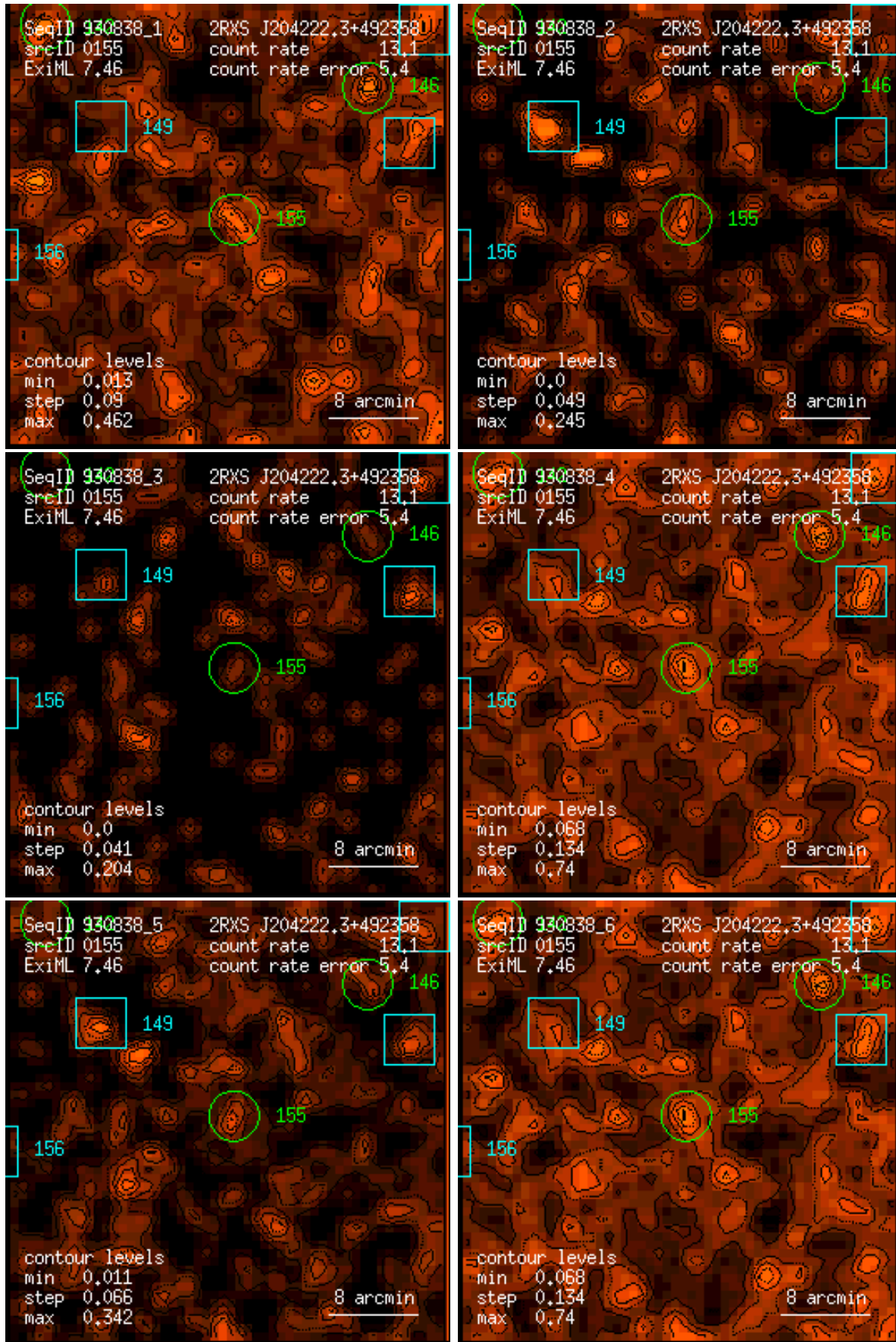
Figure 155: RASS 930838: detection 0155: band rate images, Gaussian filter: (1) PSPC channels 11 – 41, (2) 52 – 90, (3) 91 – 201, (4) 11 – 235, (5) 52 – 201, (6) 11 – 201. Broad band rates in counts/ks. Band rate contour levels in counts/ks/arcmin 2 .
