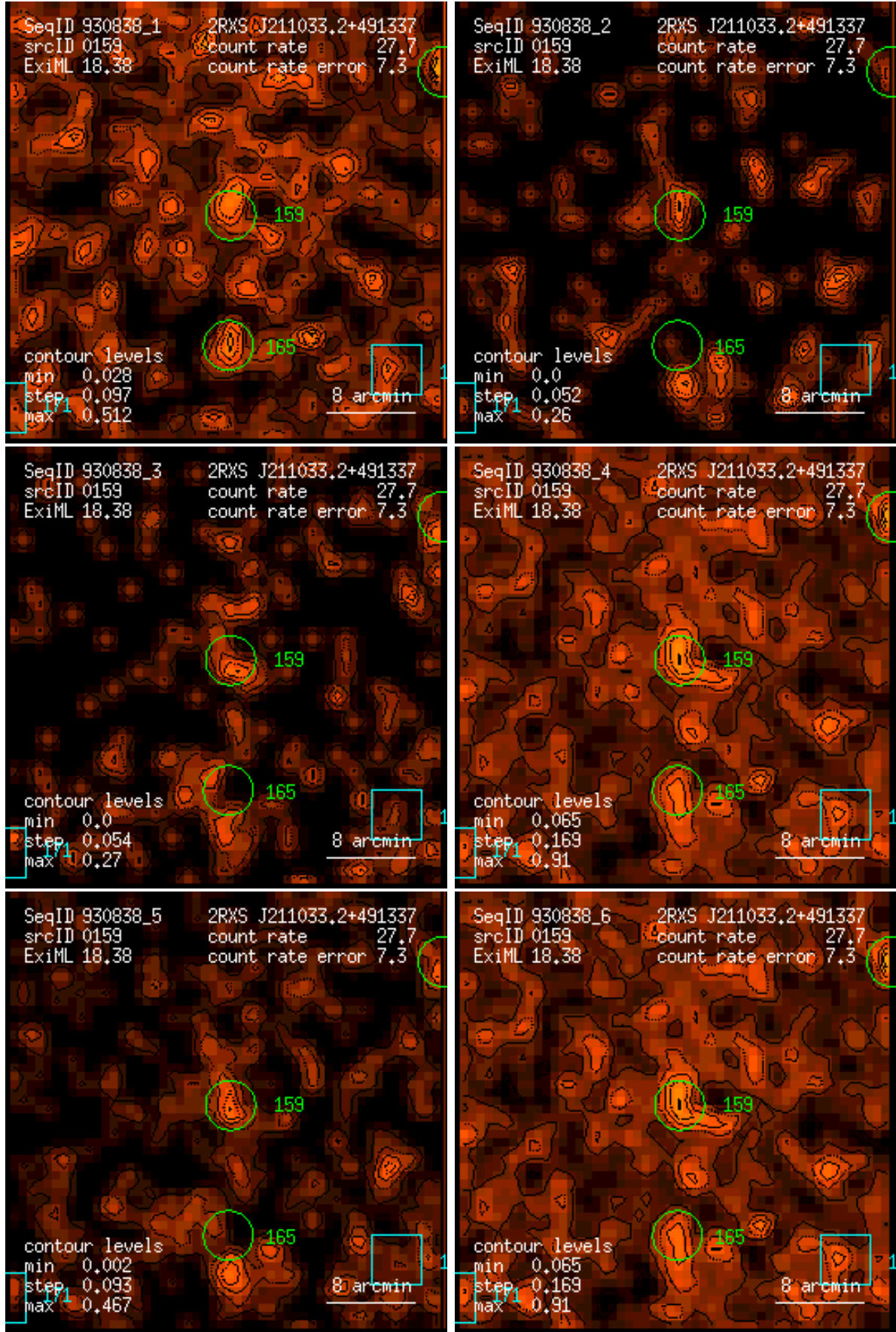
Figure 159: RASS 930838: detection 0159: band rate images, Gaussian filter: (1) PSPC channels 11 – 41, (2) 52 – 90, (3) 91 – 201, (4) 11 – 235, (5) 52 – 201, (6) 11 – 201. Broad band rates in counts/ks. Band rate contour levels in counts/ks/arcmin 2 .
