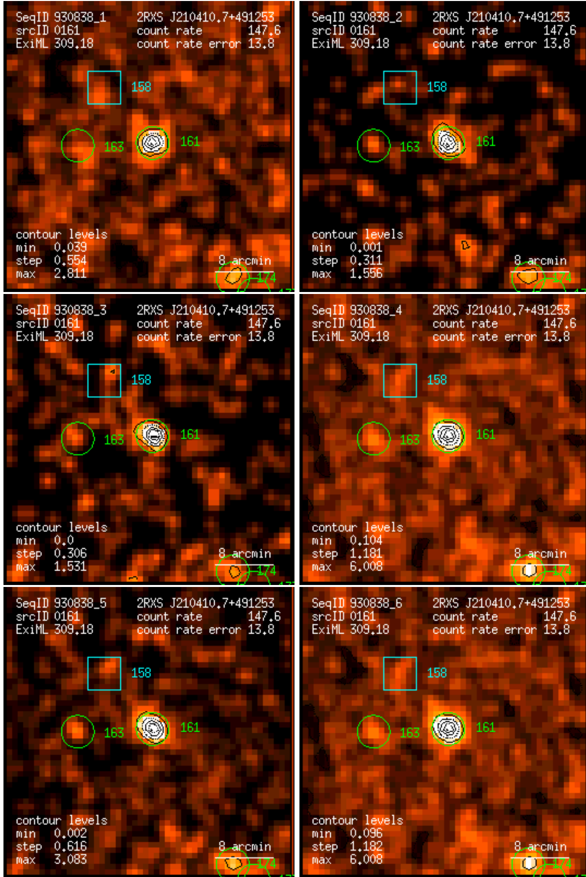
Figure 161: RASS 930838: detection 0161: band rate images, Gaussian filter: (1) PSPC channels 11 – 41, (2) 52 – 90, (3) 91 – 201, (4) 11 – 235, (5) 52 – 201, (6) 11 – 201. Broad band rates in counts/ks. Band rate contour levels in counts/ks/arcmin 2 .
