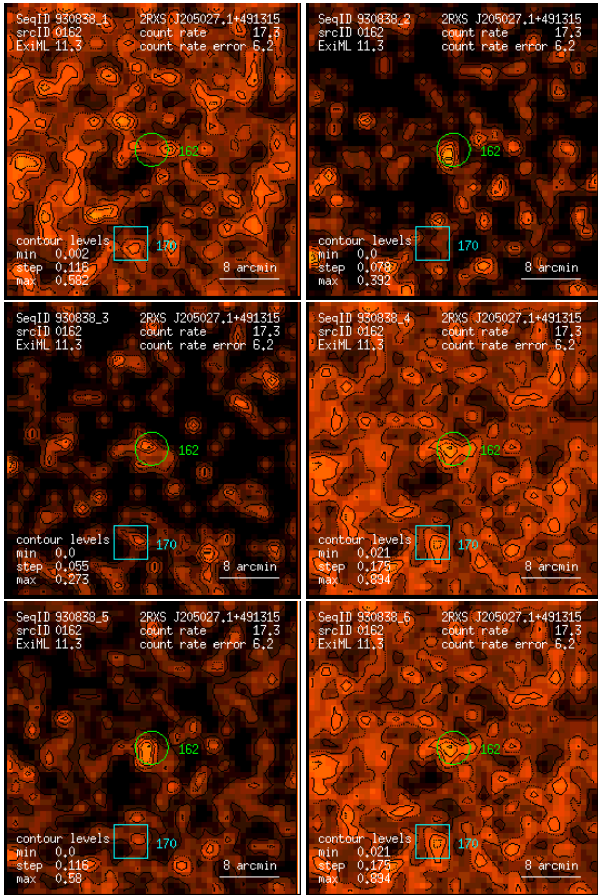
Figure 162: RASS 930838: detection 0162: band rate images, Gaussian filter: (1) PSPC channels 11 – 41, (2) 52 – 90, (3) 91 – 201, (4) 11 – 235, (5) 52 – 201, (6) 11 – 201. Broad band rates in counts/ks. Band rate contour levels in counts/ks/arcmin 2 .
