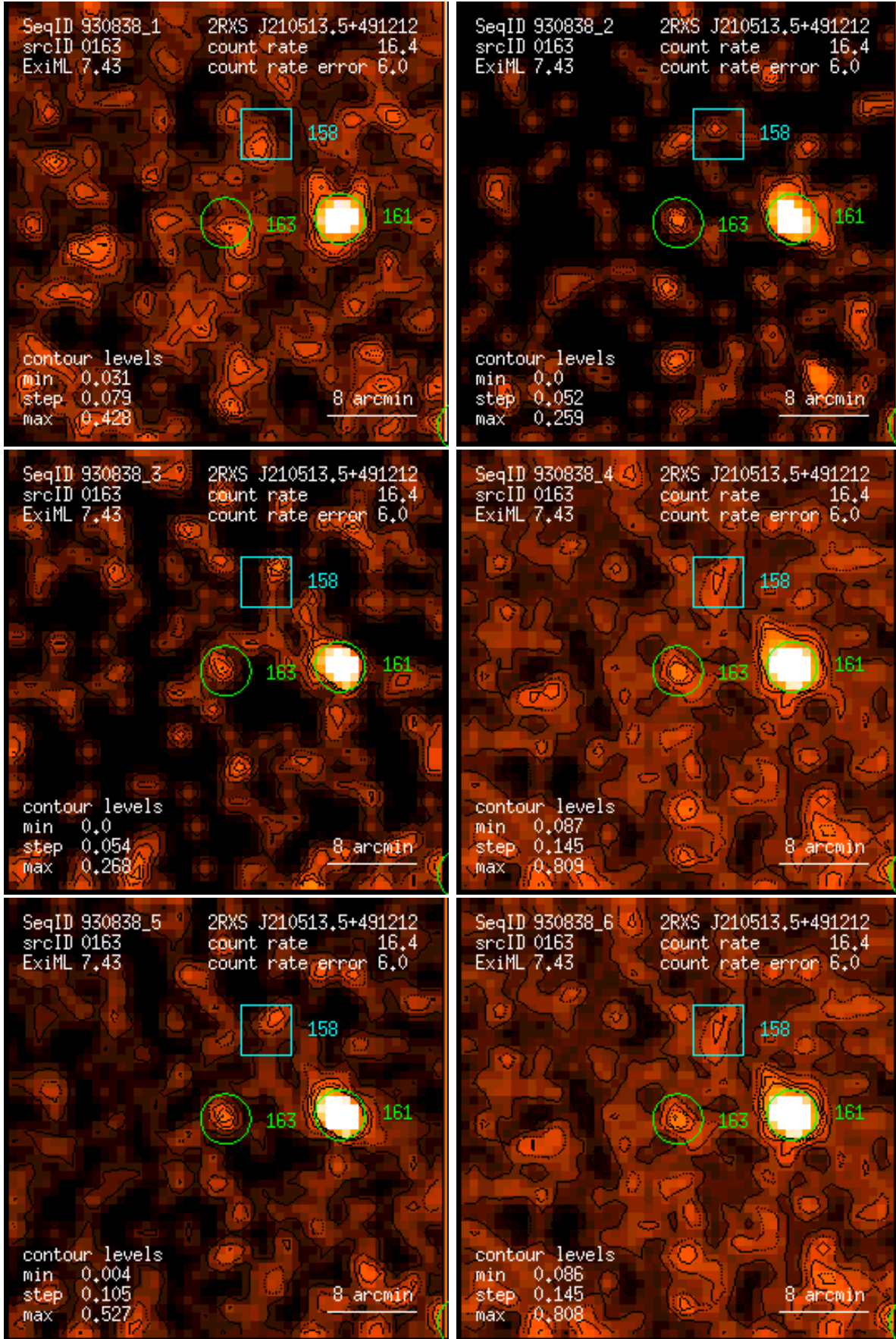
Figure 163: RASS 930838: detection 0163: band rate images, Gaussian filter: (1) PSPC channels 11 – 41, (2) 52 – 90, (3) 91 – 201, (4) 11 – 235, (5) 52 – 201, (6) 11 – 201. Broad band rates in counts/ks. Band rate contour levels in counts/ks/arcmin 2 .
