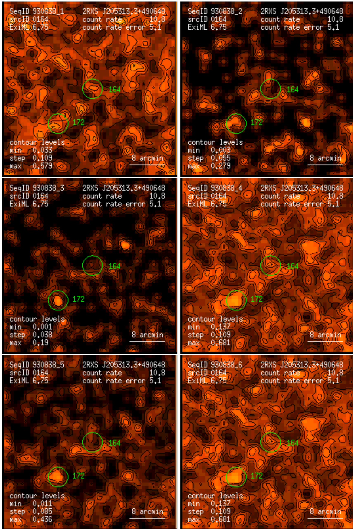
Figure 164: RASS 930838: detection 0164: band rate images, Gaussian filter: (1) PSPC channels 11 – 41, (2) 52 – 90, (3) 91 – 201, (4) 11 – 235, (5) 52 – 201, (6) 11 – 201. Broad band rates in counts/ks. Band rate contour levels in counts/ks/arcmin 2 .
