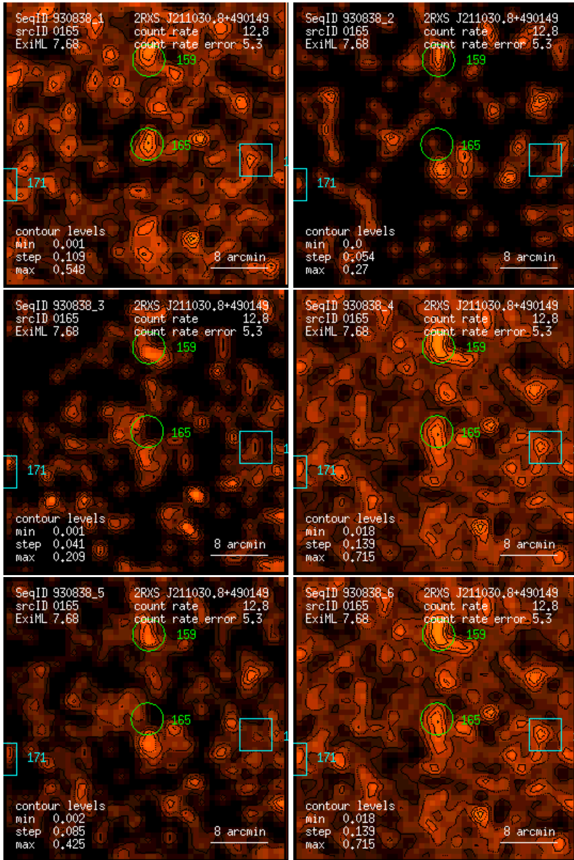
Figure 165: RASS 930838: detection 0165: band rate images, Gaussian filter: (1) PSPC channels 11 – 41, (2) 52 – 90, (3) 91 – 201, (4) 11 – 235, (5) 52 – 201, (6) 11 – 201. Broad band rates in counts/ks. Band rate contour levels in counts/ks/arcmin 2 .
