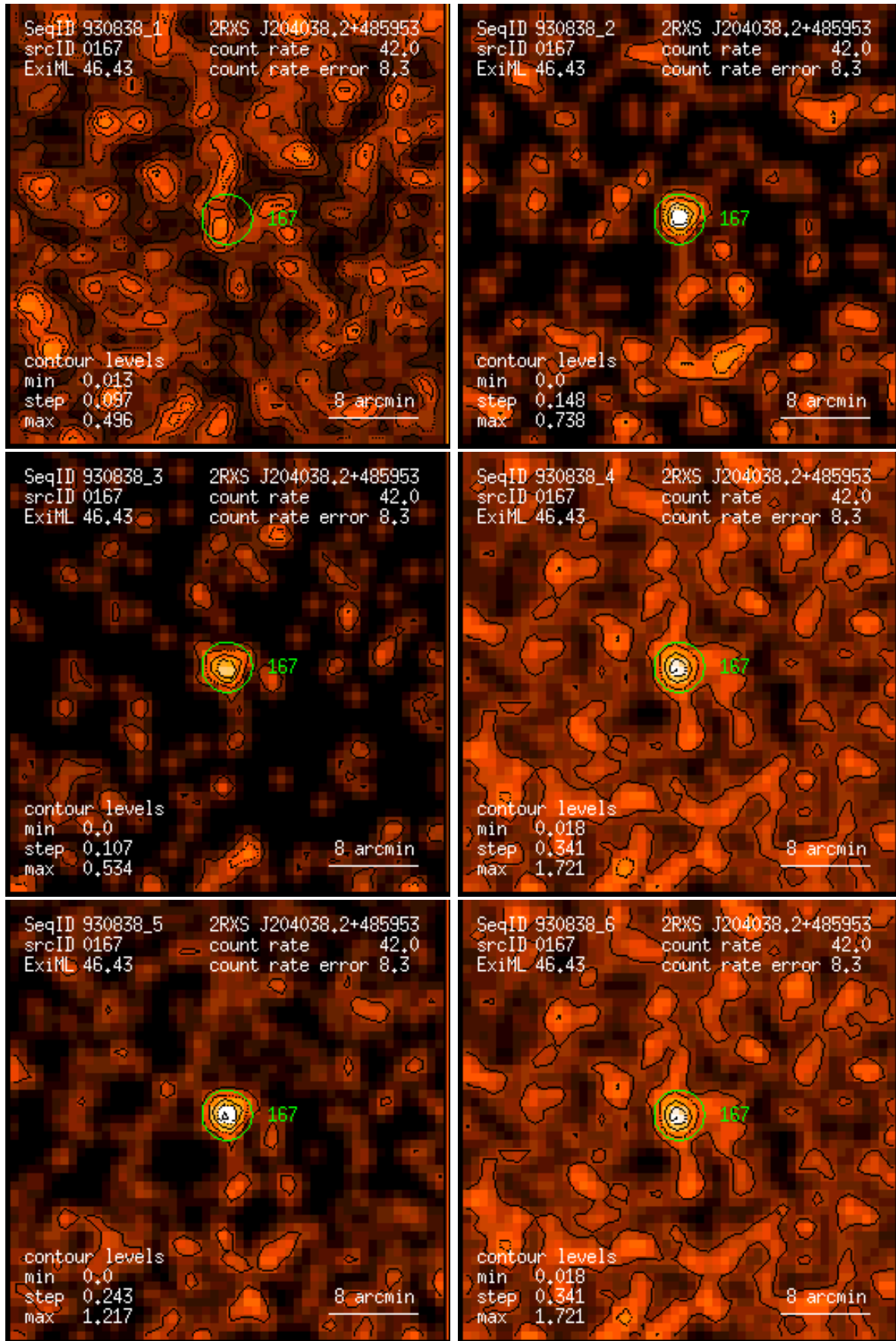
Figure 167: RASS 930838: detection 0167: band rate images, Gaussian filter: (1) PSPC channels 11 – 41, (2) 52 – 90, (3) 91 – 201, (4) 11 – 235, (5) 52 – 201, (6) 11 – 201. Broad band rates in counts/ks. Band rate contour levels in counts/ks/arcmin 2 .
