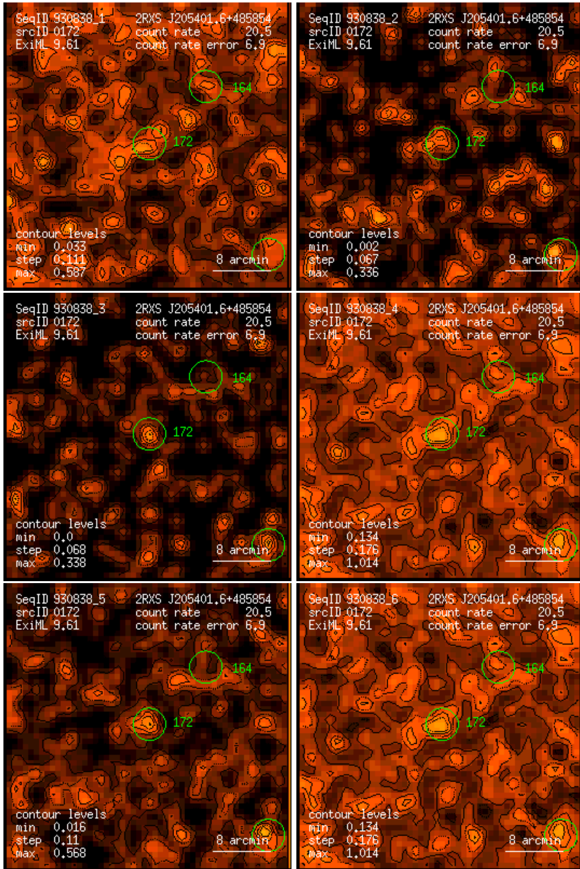
Figure 172: RASS 930838: detection 0172: band rate images, Gaussian filter: (1) PSPC channels 11 – 41, (2) 52 – 90, (3) 91 – 201, (4) 11 – 235, (5) 52 – 201, (6) 11 – 201. Broad band rates in counts/ks. Band rate contour levels in counts/ks/arcmin 2 .
