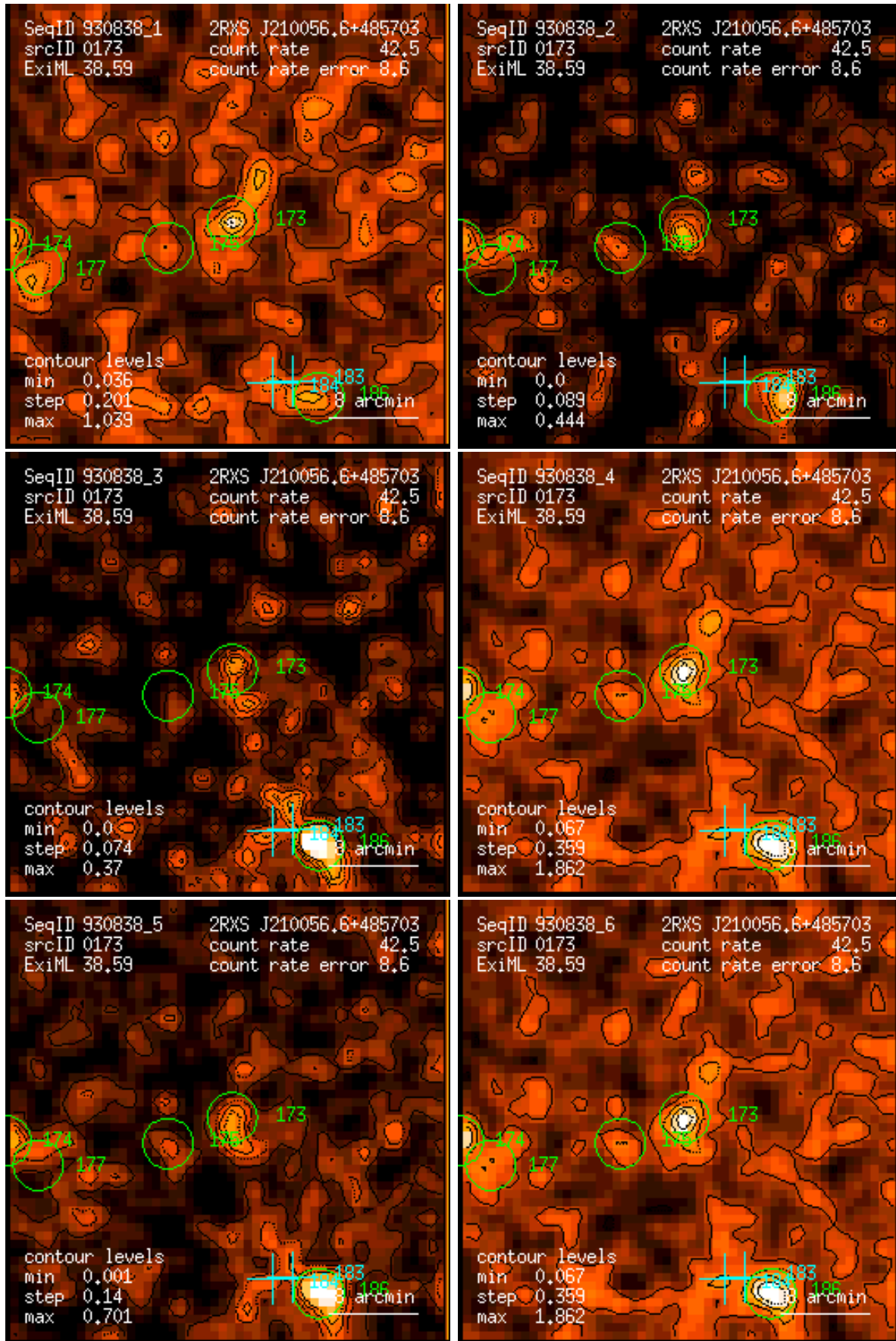
Figure 173: RASS 930838: detection 0173: band rate images, Gaussian filter: (1) PSPC channels 11 – 41, (2) 52 – 90, (3) 91 – 201, (4) 11 – 235, (5) 52 – 201, (6) 11 – 201. Broad band rates in counts/ks. Band rate contour levels in counts/ks/arcmin 2 .
