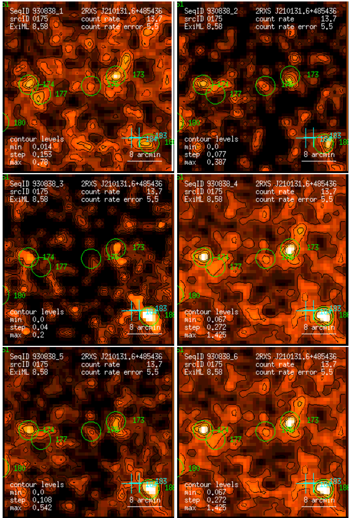
Figure 175: RASS 930838: detection 0175: band rate images, Gaussian filter: (1) PSPC channels 11 – 41, (2) 52 – 90, (3) 91 – 201, (4) 11 – 235, (5) 52 – 201, (6) 11 – 201. Broad band rates in counts/ks. Band rate contour levels in counts/ks/arcmin 2 .
