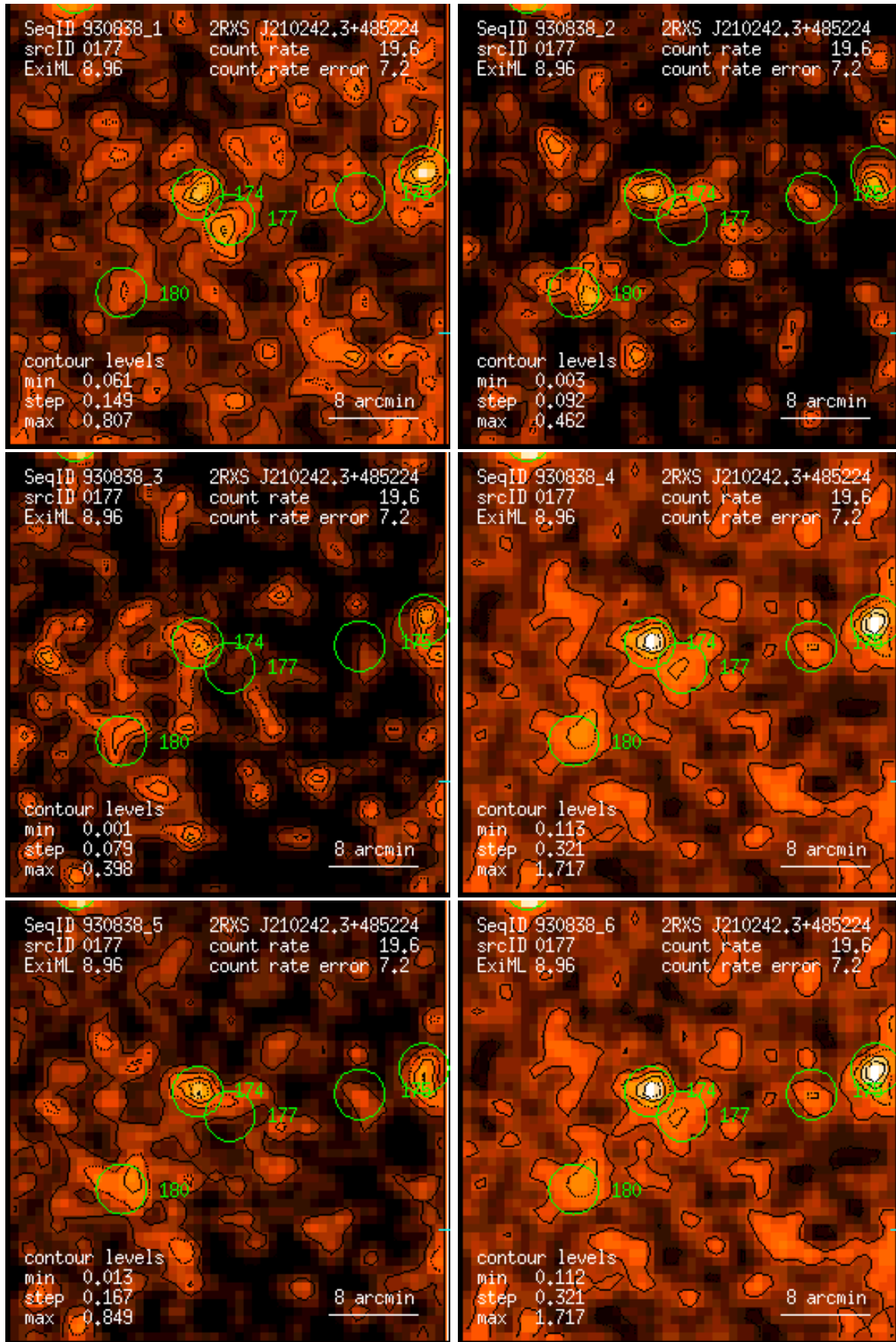
Figure 177: RASS 930838: detection 0177: band rate images, Gaussian filter: (1) PSPC channels 11 – 41, (2) 52 – 90, (3) 91 – 201, (4) 11 – 235, (5) 52 – 201, (6) 11 – 201. Broad band rates in counts/ks. Band rate contour levels in counts/ks/arcmin 2 .
