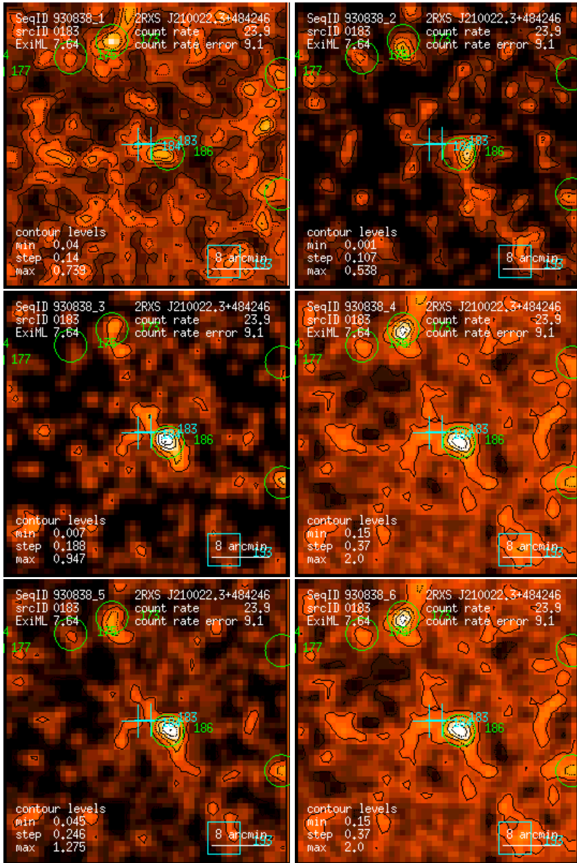
Figure 183: RASS 930838: detection 0183: band rate images, Gaussian filter: (1) PSPC channels 11 – 41, (2) 52 – 90, (3) 91 – 201, (4) 11 – 235, (5) 52 – 201, (6) 11 – 201. Broad band rates in counts/ks. Band rate contour levels in counts/ks/arcmin 2 .
