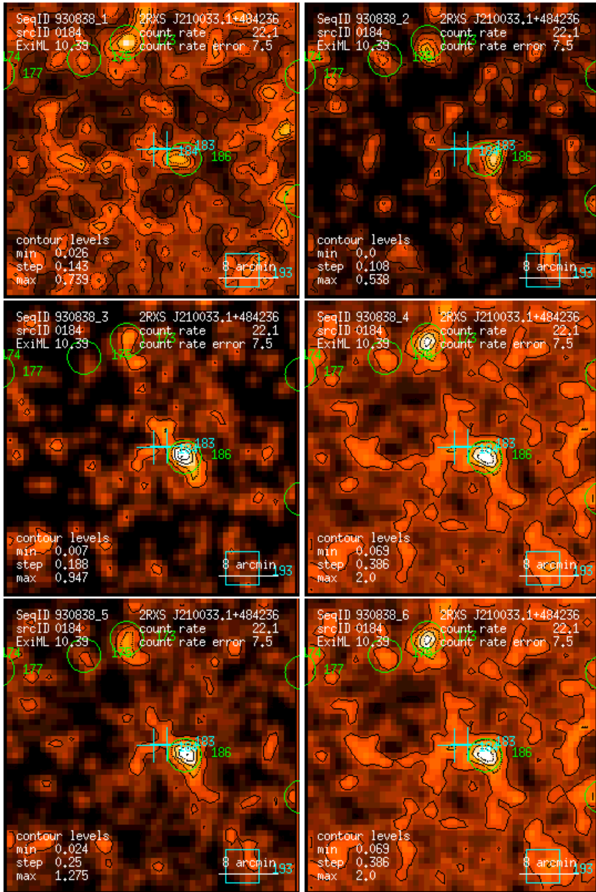
Figure 184: RASS 930838: detection 0184: band rate images, Gaussian filter: (1) PSPC channels 11 – 41, (2) 52 – 90, (3) 91 – 201, (4) 11 – 235, (5) 52 – 201, (6) 11 – 201. Broad band rates in counts/ks. Band rate contour levels in counts/ks/arcmin 2 .
