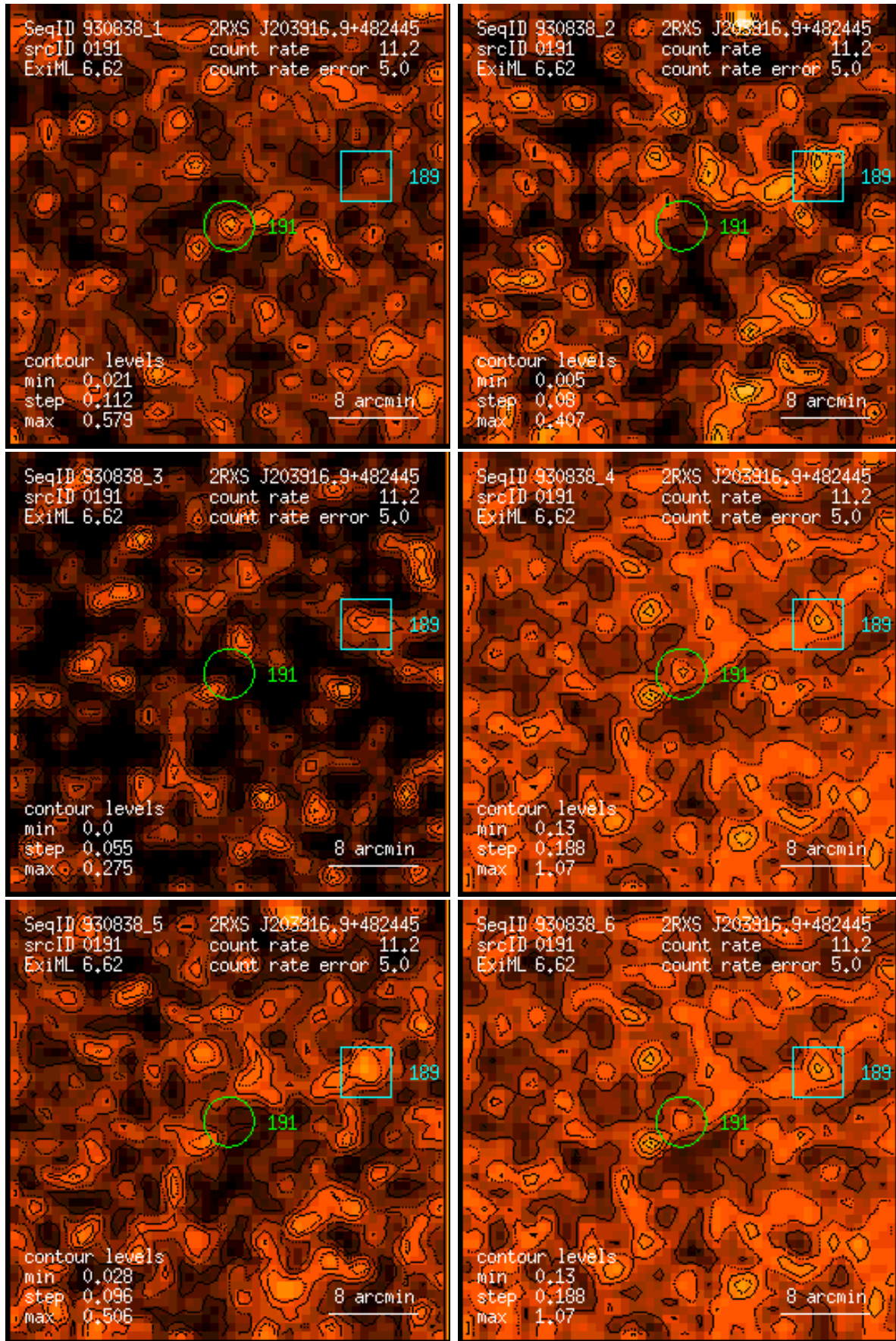
Figure 191: RASS 930838: detection 0191: band rate images, Gaussian filter: (1) PSPC channels 11 – 41, (2) 52 – 90, (3) 91 – 201, (4) 11 – 235, (5) 52 – 201, (6) 11 – 201. Broad band rates in counts/ks. Band rate contour levels in counts/ks/arcmin 2 .
