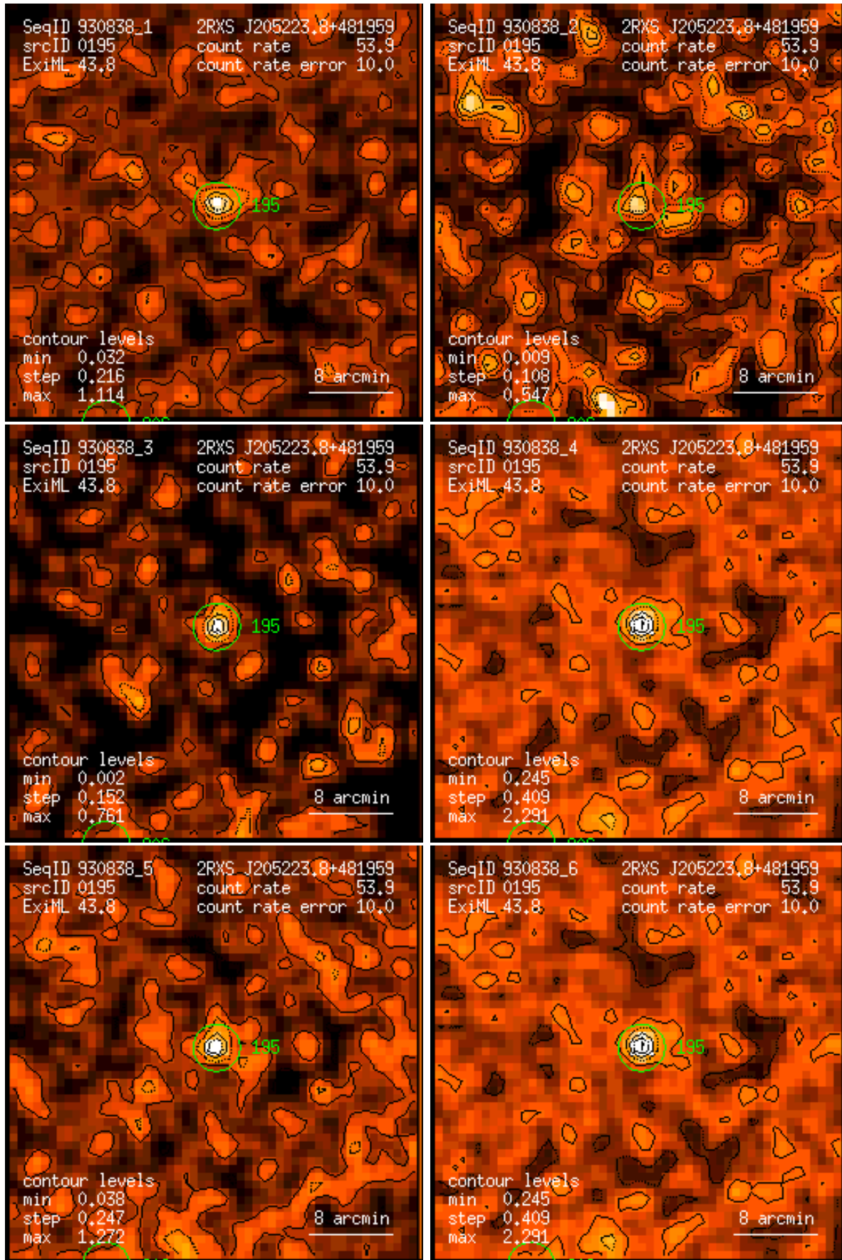
Figure 195: RASS 930838: detection 0195: band rate images, Gaussian filter: (1) PSPC channels 11 – 41, (2) 52 – 90, (3) 91 – 201, (4) 11 – 235, (5) 52 – 201, (6) 11 – 201. Broad band rates in counts/ks. Band rate contour levels in counts/ks/arcmin 2 .
