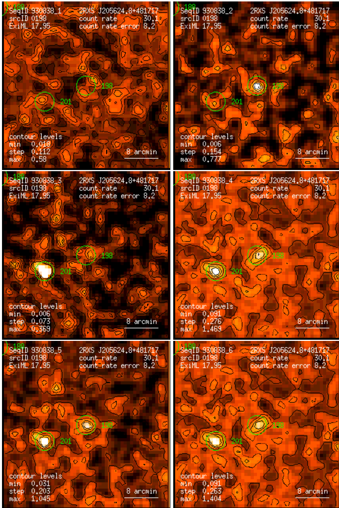
Figure 198: RASS 930838: detection 0198: band rate images, Gaussian filter: (1) PSPC channels 11 – 41, (2) 52 – 90, (3) 91 – 201, (4) 11 – 235, (5) 52 – 201, (6) 11 – 201. Broad band rates in counts/ks. Band rate contour levels in counts/ks/arcmin 2 .
