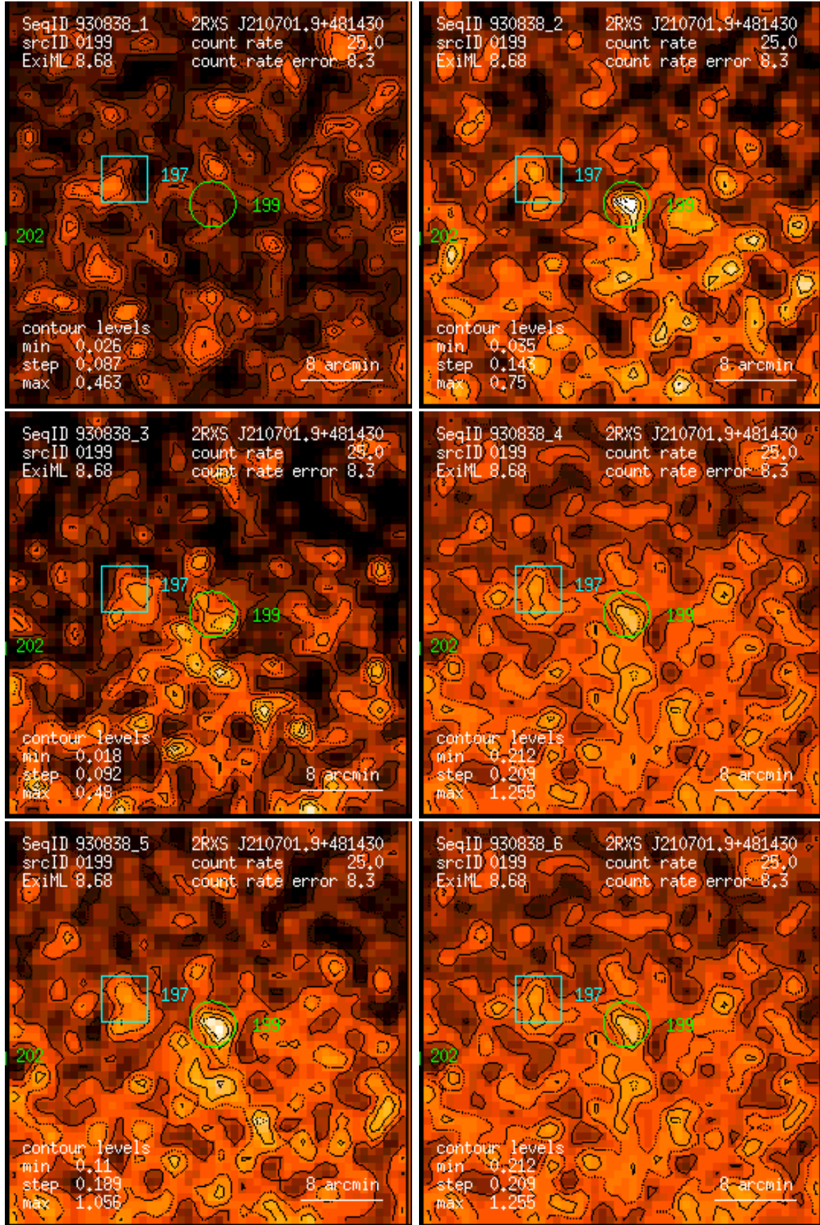
Figure 199: RASS 930838: detection 0199: band rate images, Gaussian filter: (1) PSPC channels 11 – 41, (2) 52 – 90, (3) 91 – 201, (4) 11 – 235, (5) 52 – 201, (6) 11 – 201. Broad band rates in counts/ks. Band rate contour levels in counts/ks/arcmin 2 .
