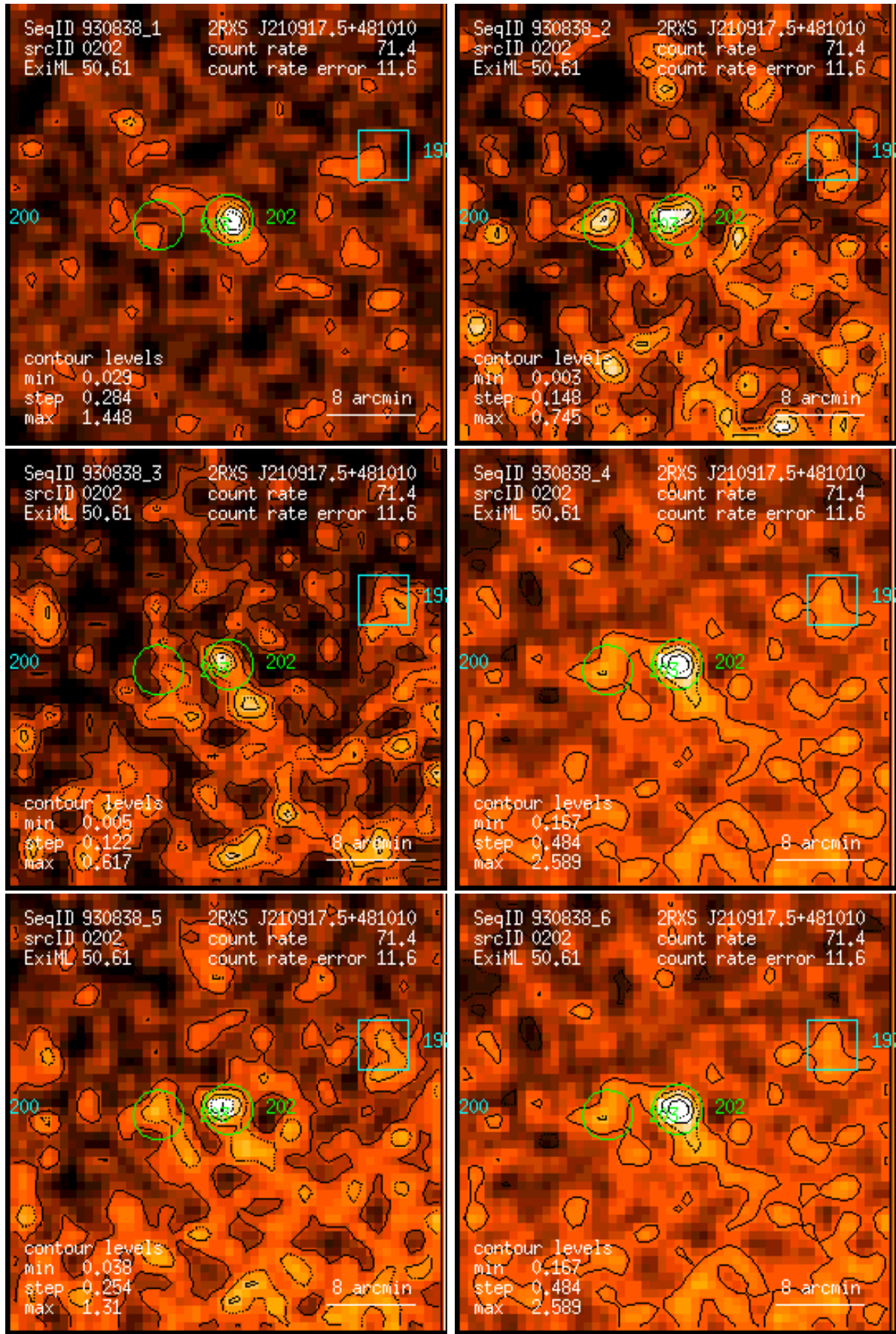
Figure 202: RASS 930838: detection 0202: band rate images, Gaussian filter: (1) PSPC channels 11 – 41, (2) 52 – 90, (3) 91 – 201, (4) 11 – 235, (5) 52 – 201, (6) 11 – 201. Broad band rates in counts/ks. Band rate contour levels in counts/ks/arcmin 2 .
