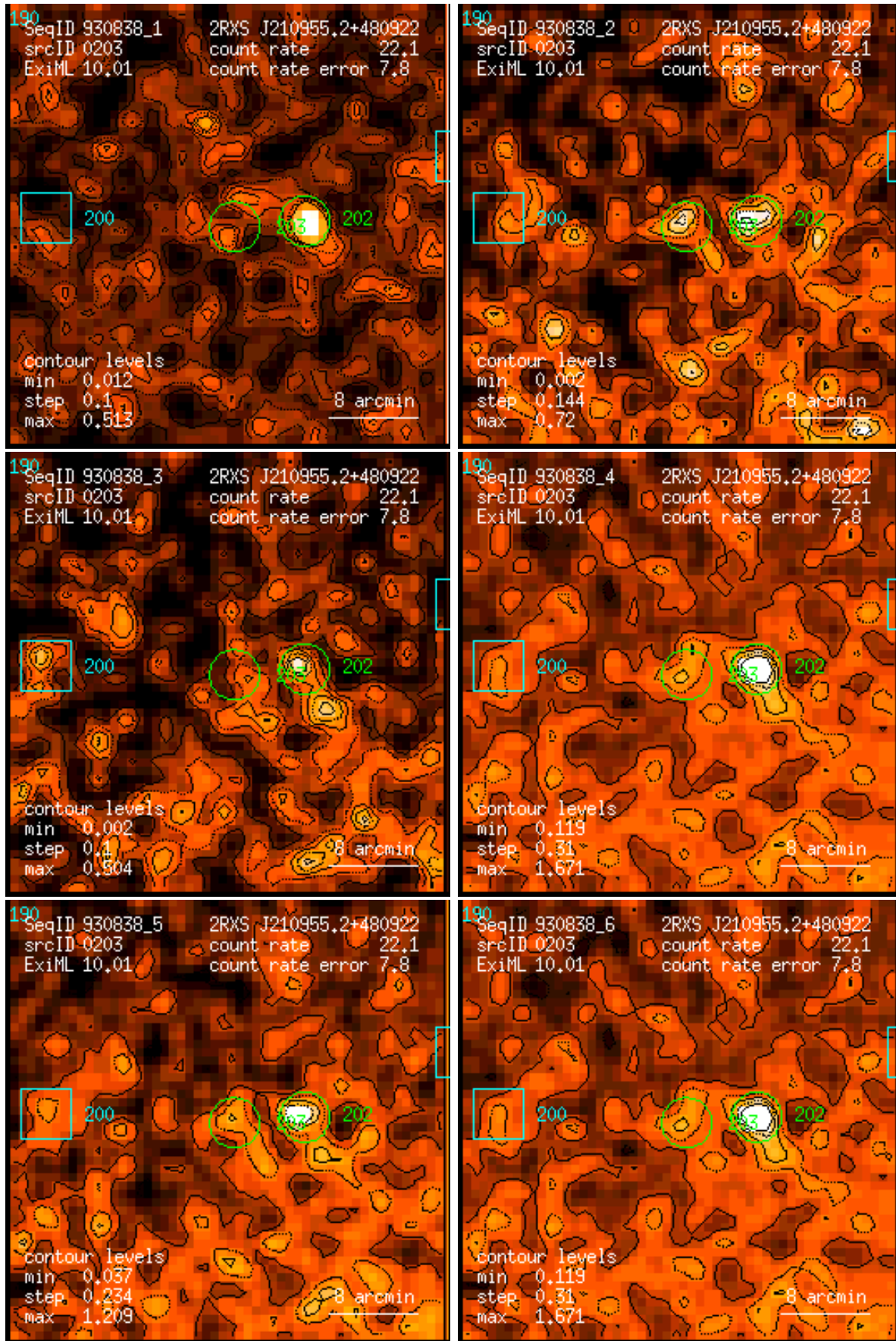
Figure 203: RASS 930838: detection 0203: band rate images, Gaussian filter: (1) PSPC channels 11 – 41, (2) 52 – 90, (3) 91 – 201, (4) 11 – 235, (5) 52 – 201, (6) 11 – 201. Broad band rates in counts/ks. Band rate contour levels in counts/ks/arcmin 2 .
