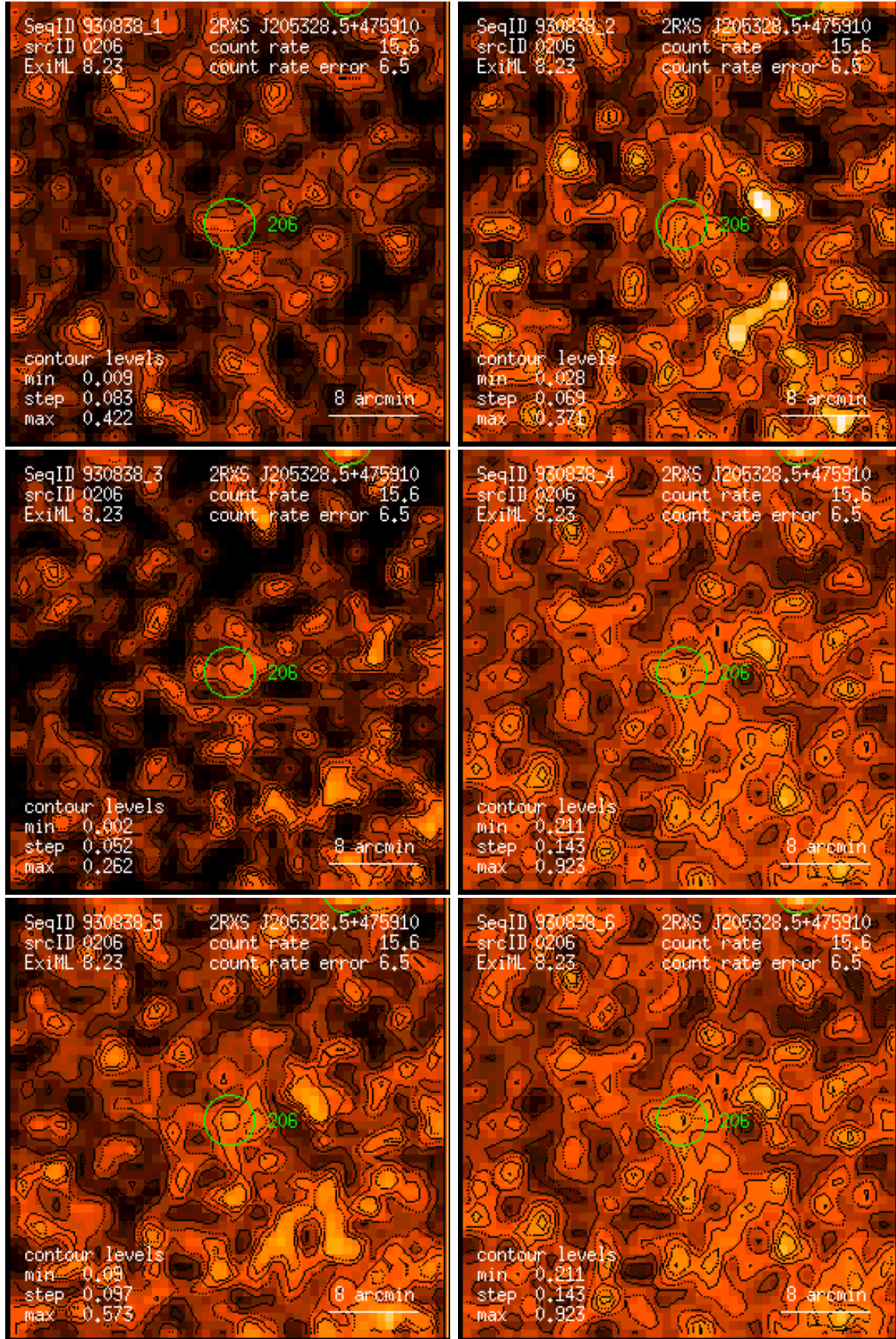
Figure 206: RASS 930838: detection 0206: band rate images, Gaussian filter: (1) PSPC channels 11 – 41, (2) 52 – 90, (3) 91 – 201, (4) 11 – 235, (5) 52 – 201, (6) 11 – 201. Broad band rates in counts/ks. Band rate contour levels in counts/ks/arcmin 2 .
