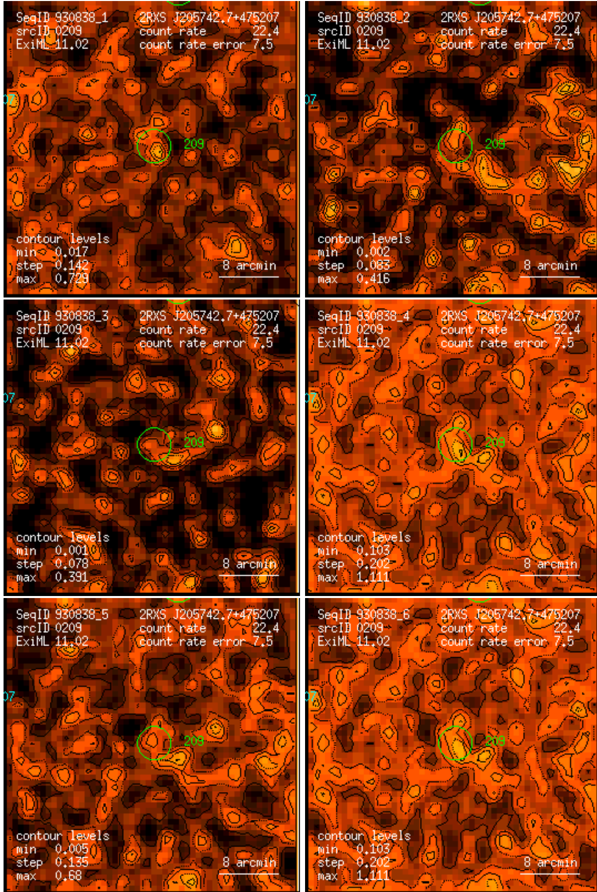
Figure 209: RASS 930838: detection 0209: band rate images, Gaussian filter: (1) PSPC channels 11 – 41, (2) 52 – 90, (3) 91 – 201, (4) 11 – 235, (5) 52 – 201, (6) 11 – 201. Broad band rates in counts/ks. Band rate contour levels in counts/ks/arcmin 2 .
