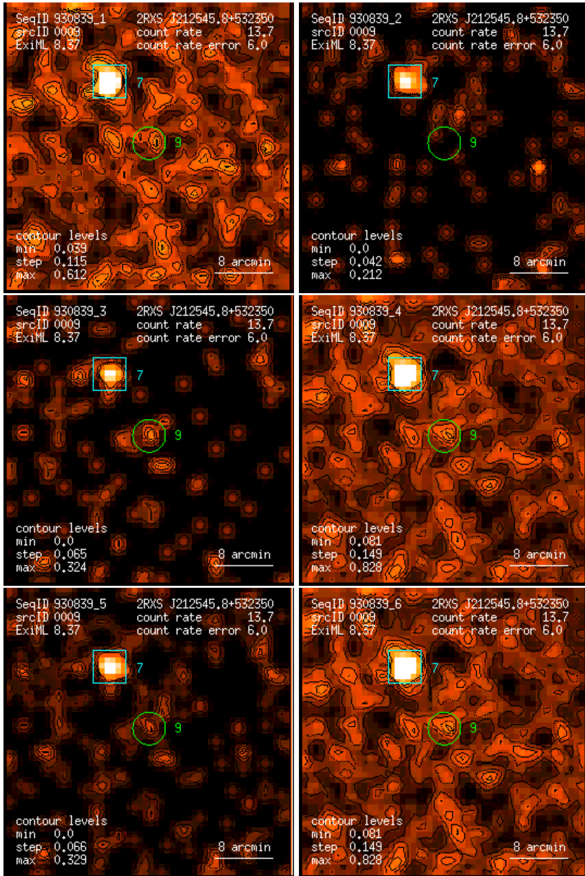
Figure 9: RASS 930839: detection 0009: band rate images, Gaussian filter: (1) PSPC channels 11 – 41, (2) 52 – 90, (3) 91 – 201, (4) 11 – 235, (5) 52 – 201, (6) 11 – 201. Broad band rates in counts/ks. Band rate contour levels in counts/ks/arcmin 2 .
