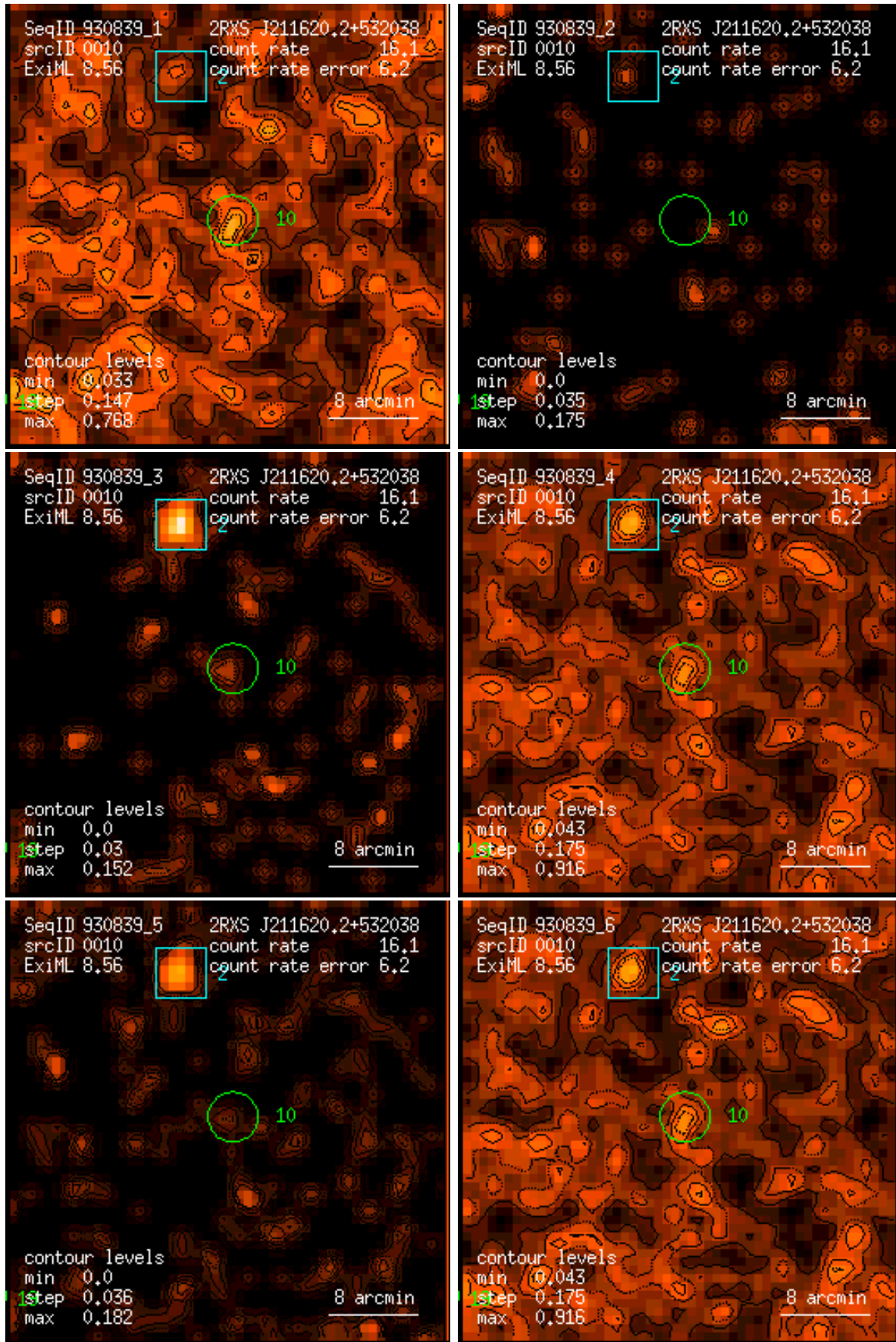
Figure 10: RASS 930839: detection 0010: band rate images, Gaussian filter: (1) PSPC channels 11 – 41, (2) 52 – 90, (3) 91 – 201, (4) 11 – 235, (5) 52 – 201, (6) 11 – 201. Broad band rates in counts/ks. Band rate contour levels in counts/ks/arcmin 2 .
