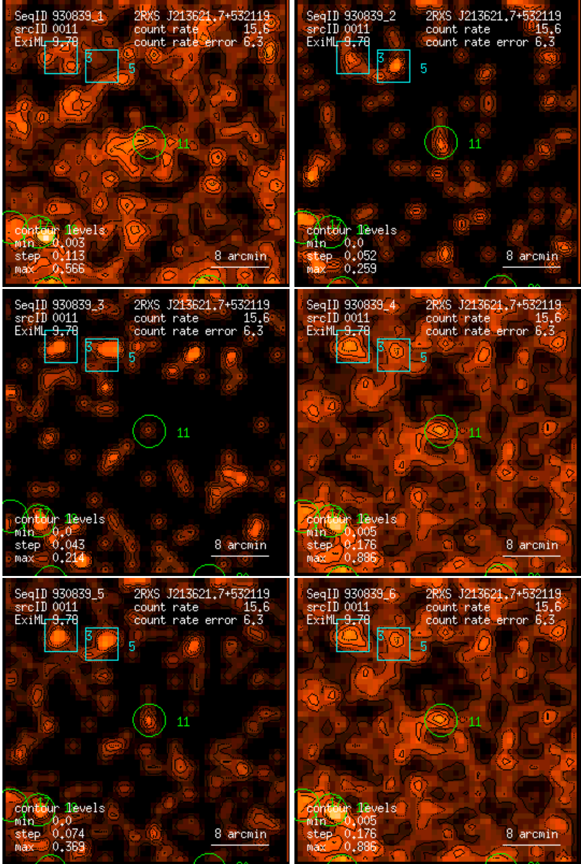
Figure 11: RASS 930839: detection 0011: band rate images, Gaussian filter: (1) PSPC channels 11 – 41, (2) 52 – 90, (3) 91 – 201, (4) 11 – 235, (5) 52 – 201, (6) 11 – 201. Broad band rates in counts/ks. Band rate contour levels in counts/ks/arcmin 2 .
