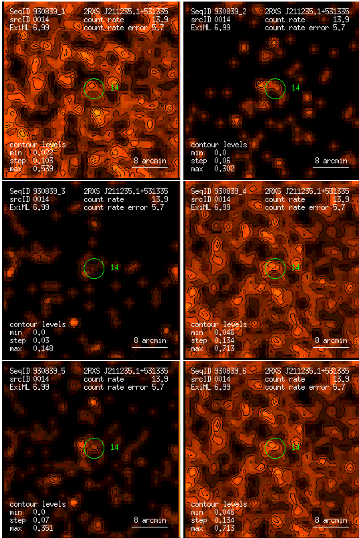
Figure 14: RASS 930839: detection 0014: band rate images, Gaussian filter: (1) PSPC channels 11 – 41, (2) 52 – 90, (3) 91 – 201, (4) 11 – 235, (5) 52 – 201, (6) 11 – 201. Broad band rates in counts/ks. Band rate contour levels in counts/ks/arcmin 2 .
