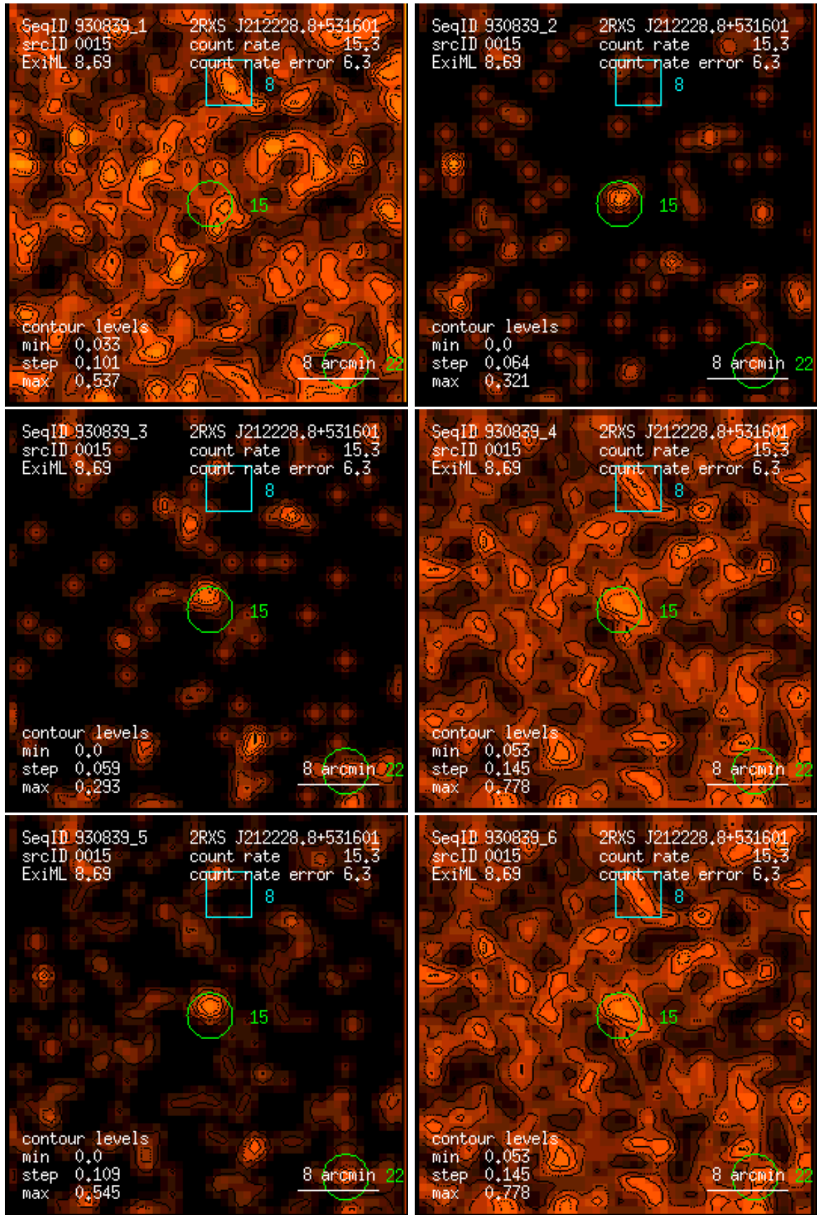
Figure 15: RASS 930839: detection 0015: band rate images, Gaussian filter: (1) PSPC channels 11 – 41, (2) 52 – 90, (3) 91 – 201, (4) 11 – 235, (5) 52 – 201, (6) 11 – 201. Broad band rates in counts/ks. Band rate contour levels in counts/ks/arcmin 2 .
