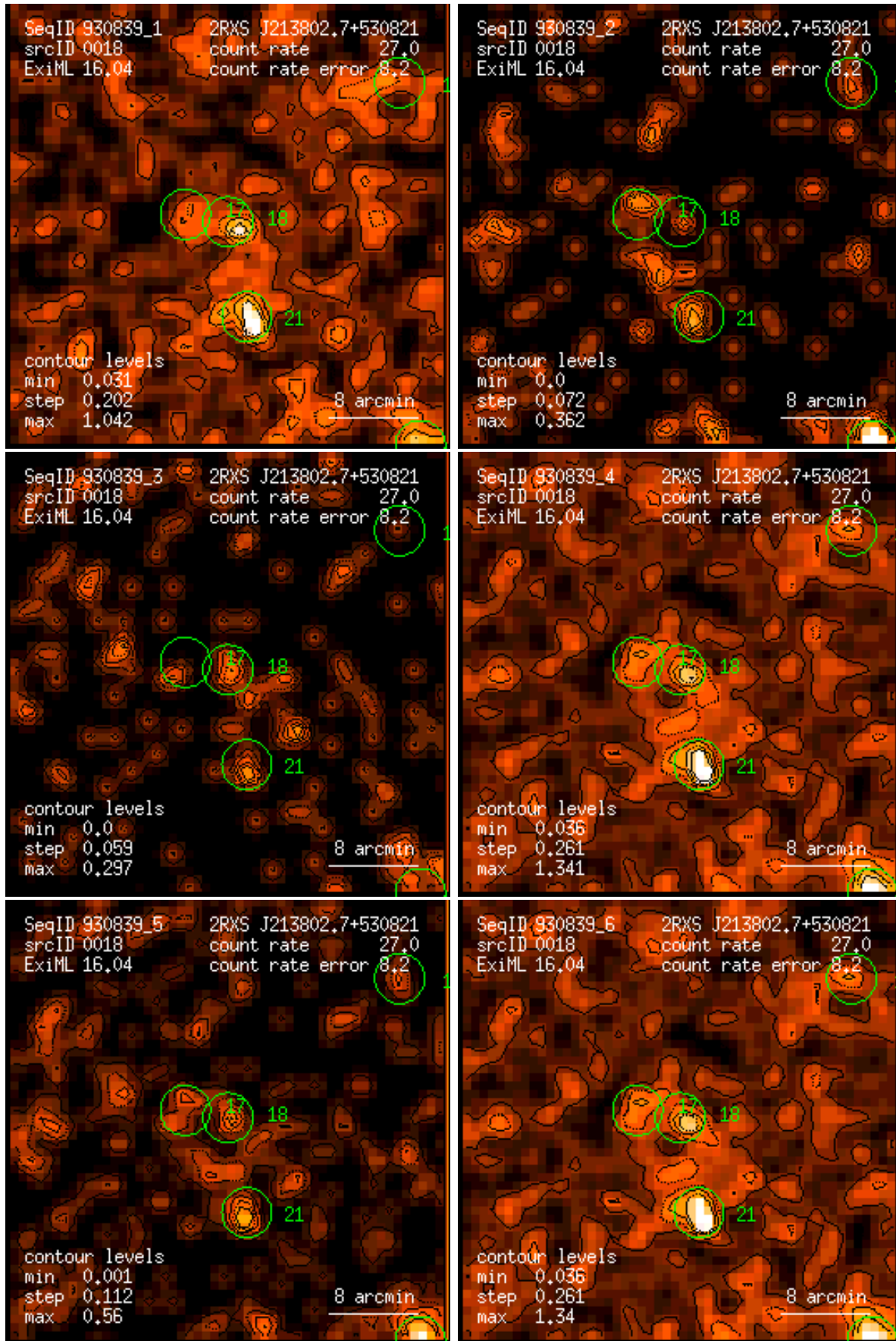
Figure 18: RASS 930839: detection 0018: band rate images, Gaussian filter: (1) PSPC channels 11 – 41, (2) 52 – 90, (3) 91 – 201, (4) 11 – 235, (5) 52 – 201, (6) 11 – 201. Broad band rates in counts/ks. Band rate contour levels in counts/ks/arcmin 2 .
