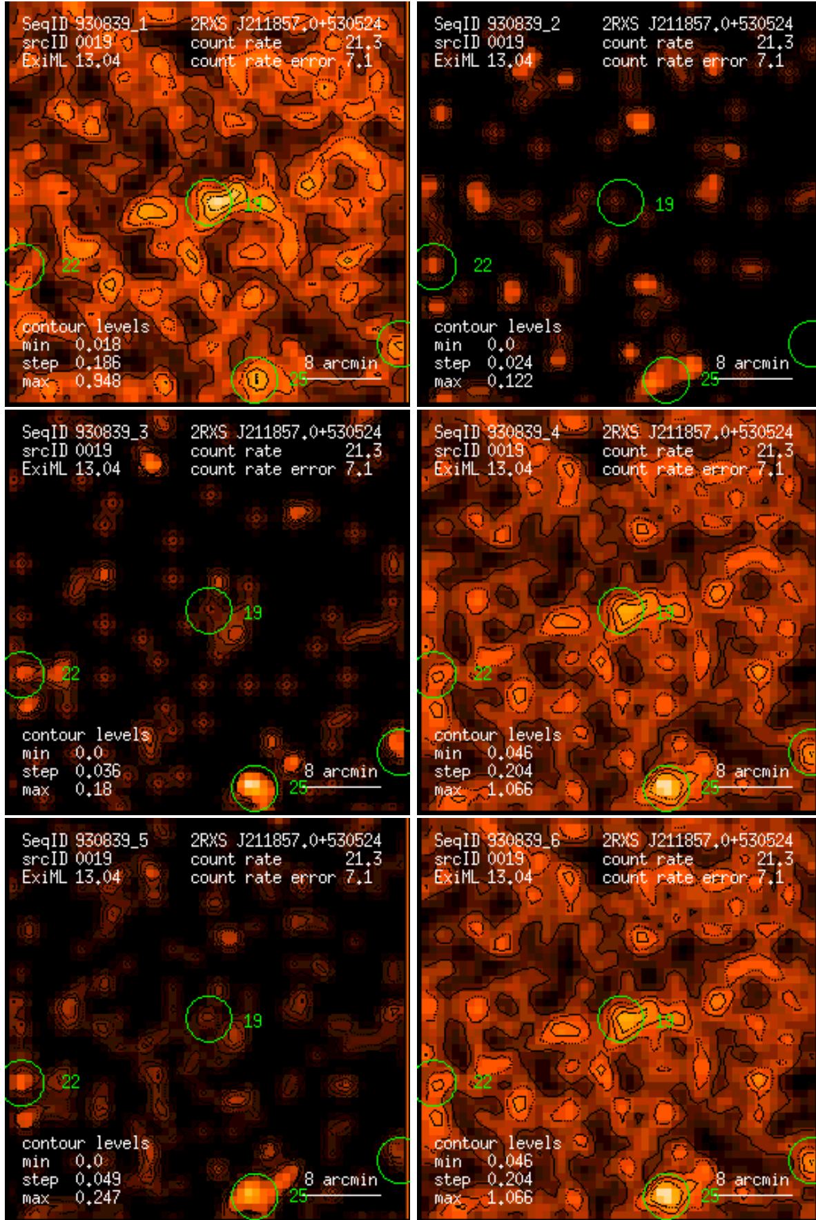
Figure 19: RASS 930839: detection 0019: band rate images, Gaussian filter: (1) PSPC channels 11 – 41, (2) 52 – 90, (3) 91 – 201, (4) 11 – 235, (5) 52 – 201, (6) 11 – 201. Broad band rates in counts/ks. Band rate contour levels in counts/ks/arcmin 2 .
