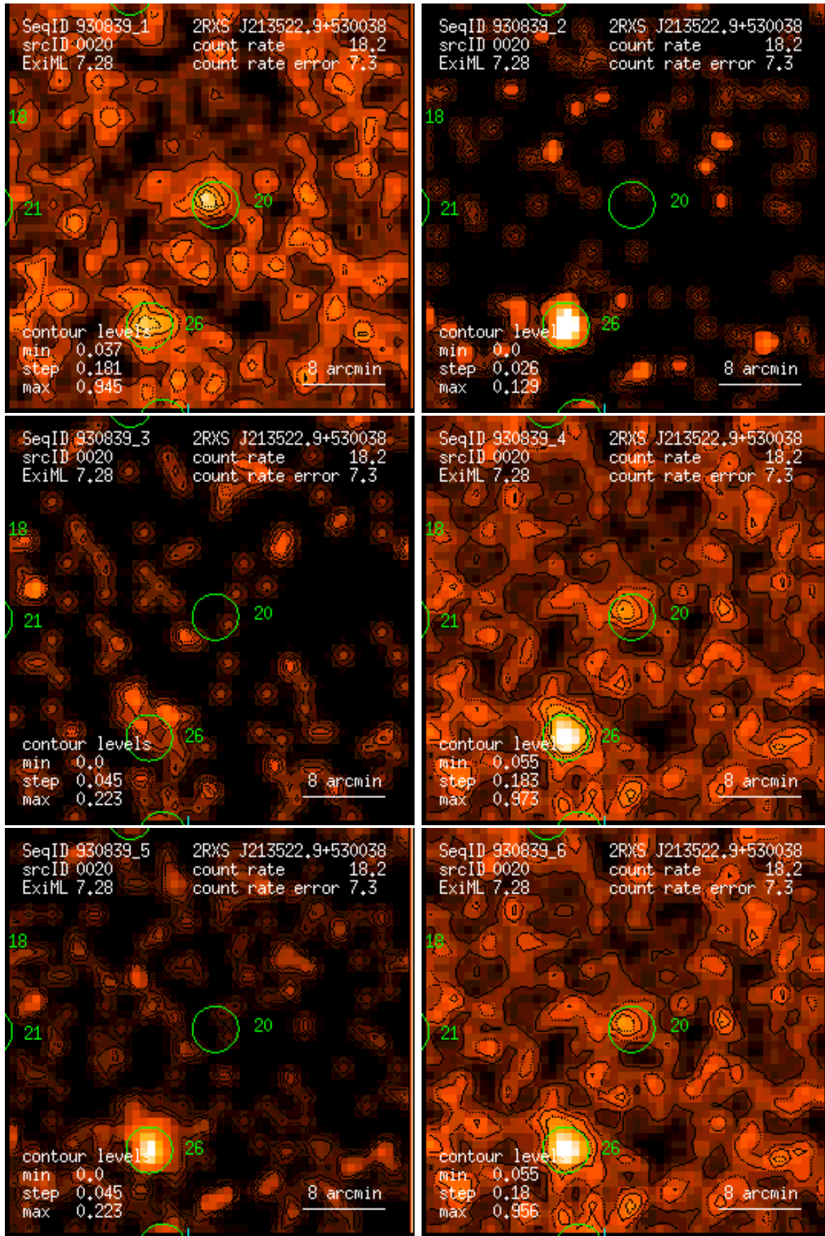
Figure 20: RASS 930839: detection 0020: band rate images, Gaussian filter: (1) PSPC channels 11 – 41, (2) 52 – 90, (3) 91 – 201, (4) 11 – 235, (5) 52 – 201, (6) 11 – 201. Broad band rates in counts/ks. Band rate contour levels in counts/ks/arcmin 2 .
