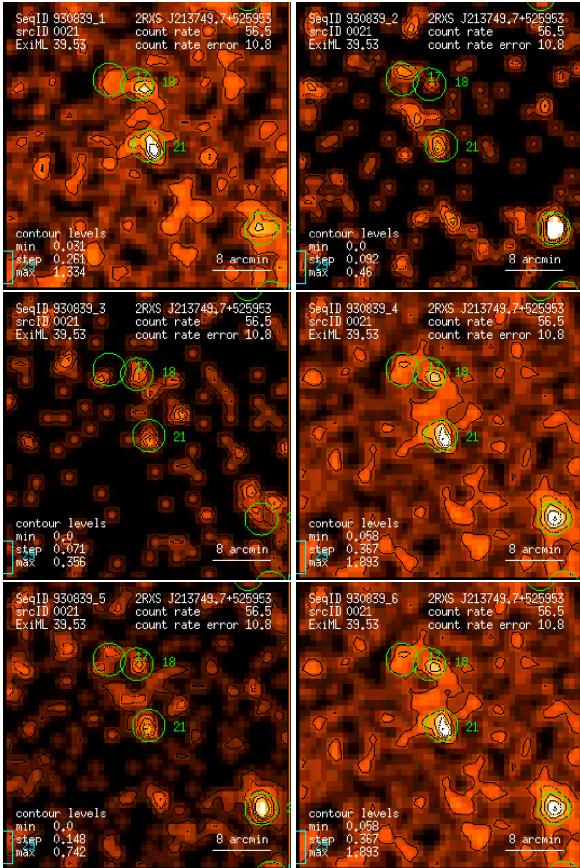
Figure 21: RASS 930839: detection 0021: band rate images, Gaussian filter: (1) PSPC channels 11 – 41, (2) 52 – 90, (3) 91 – 201, (4) 11 – 235, (5) 52 – 201, (6) 11 – 201. Broad band rates in counts/ks. Band rate contour levels in counts/ks/arcmin 2 .
