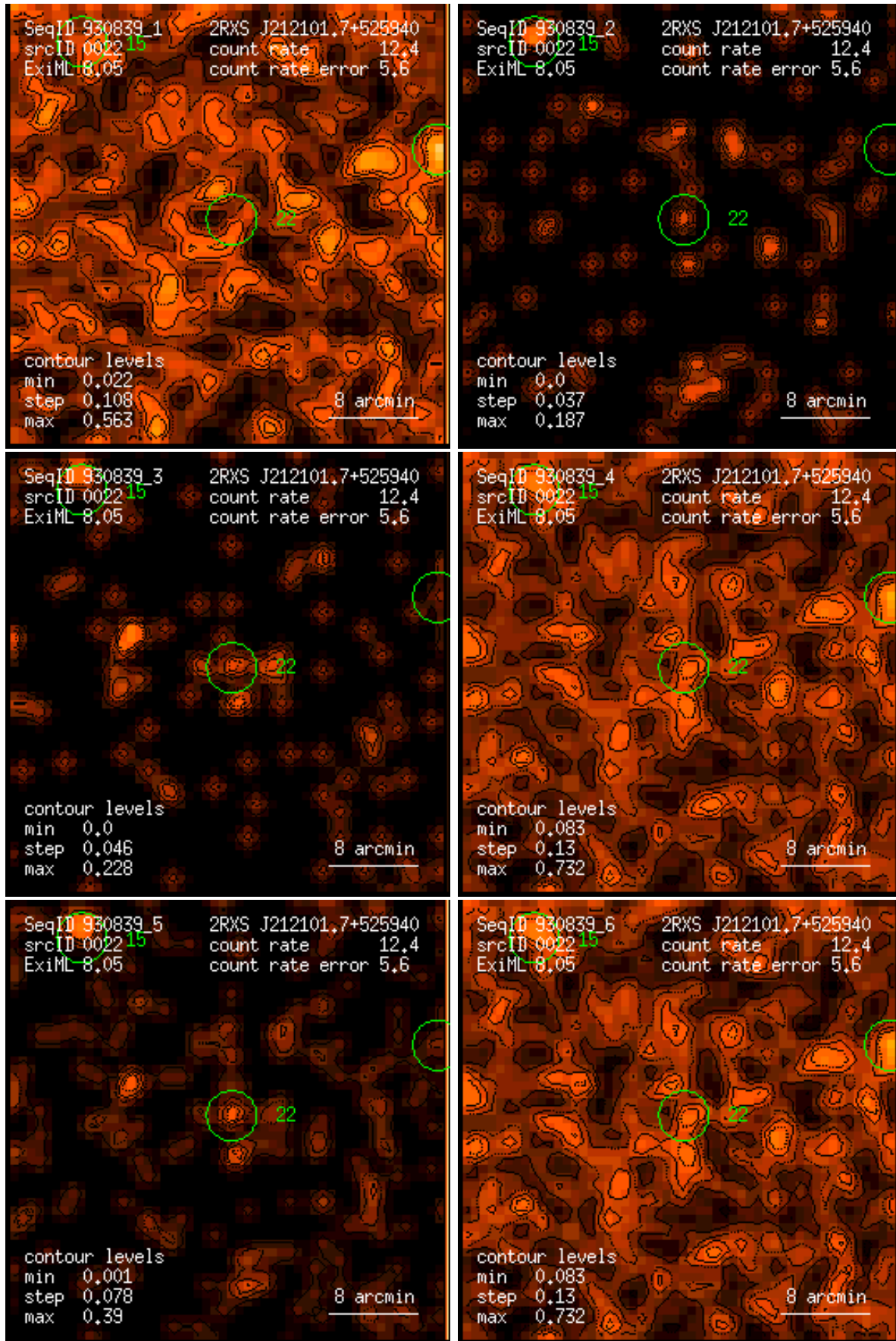
Figure 22: RASS 930839: detection 0022: band rate images, Gaussian filter: (1) PSPC channels 11 – 41, (2) 52 – 90, (3) 91 – 201, (4) 11 – 235, (5) 52 – 201, (6) 11 – 201. Broad band rates in counts/ks. Band rate contour levels in counts/ks/arcmin 2 .
