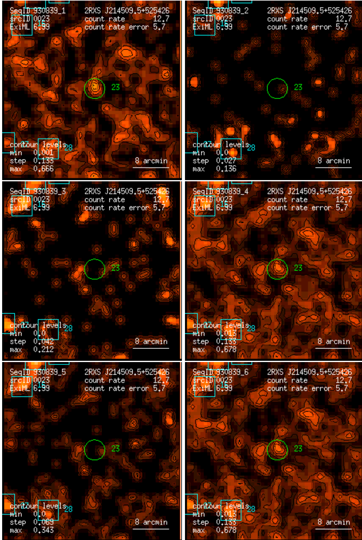
Figure 23: RASS 930839: detection 0023: band rate images, Gaussian filter: (1) PSPC channels 11 – 41, (2) 52 – 90, (3) 91 – 201, (4) 11 – 235, (5) 52 – 201, (6) 11 – 201. Broad band rates in counts/ks. Band rate contour levels in counts/ks/arcmin 2 .
