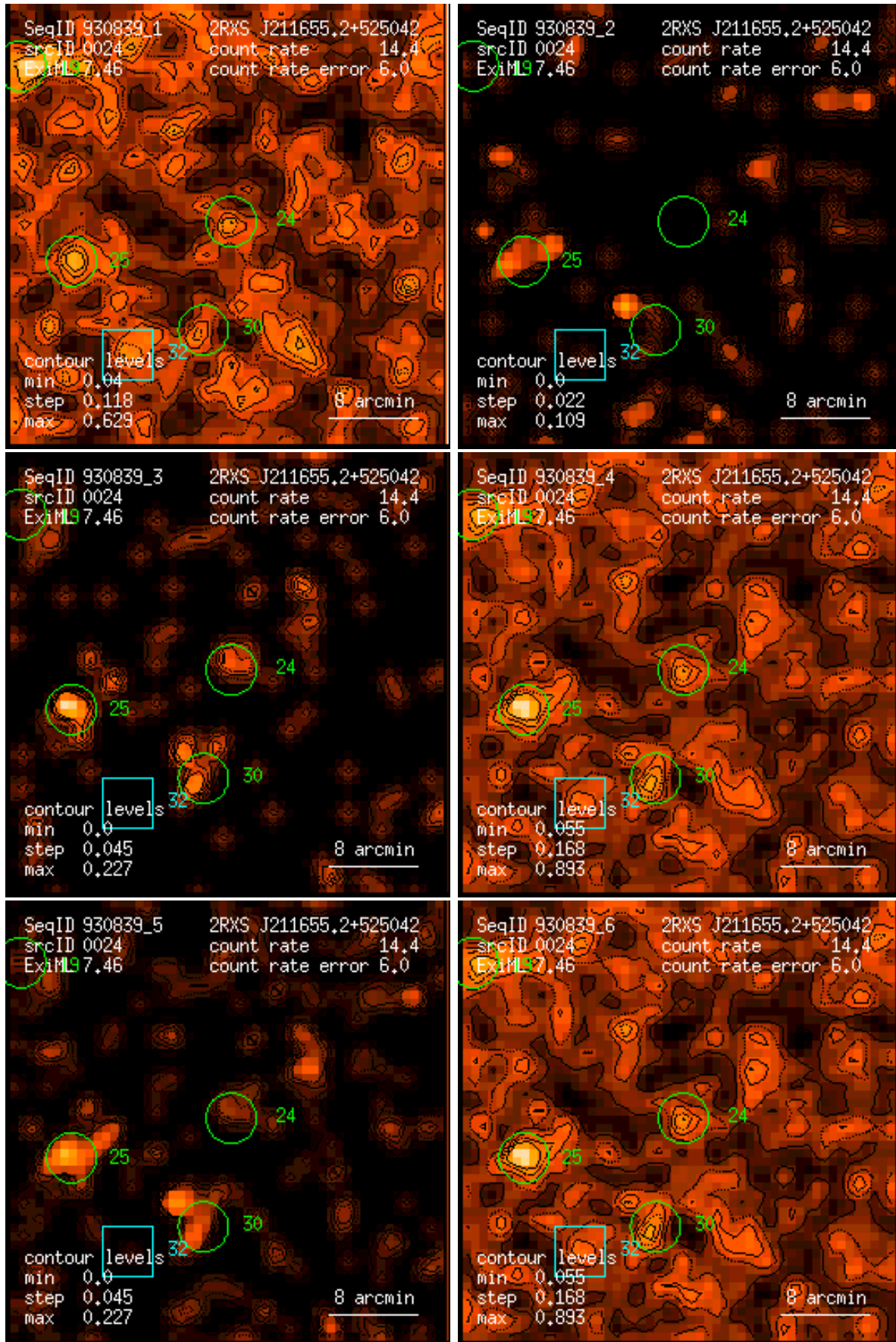
Figure 24: RASS 930839: detection 0024: band rate images, Gaussian filter: (1) PSPC channels 11 – 41, (2) 52 – 90, (3) 91 – 201, (4) 11 – 235, (5) 52 – 201, (6) 11 – 201. Broad band rates in counts/ks. Band rate contour levels in counts/ks/arcmin 2 .
