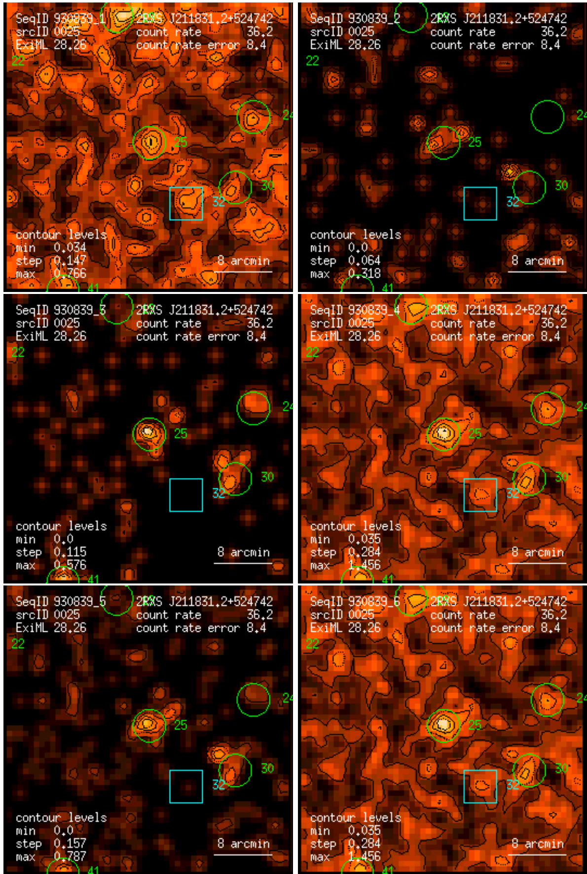
Figure 25: RASS 930839: detection 0025: band rate images, Gaussian filter: (1) PSPC channels 11 – 41, (2) 52 – 90, (3) 91 – 201, (4) 11 – 235, (5) 52 – 201, (6) 11 – 201. Broad band rates in counts/ks. Band rate contour levels in counts/ks/arcmin 2 .
