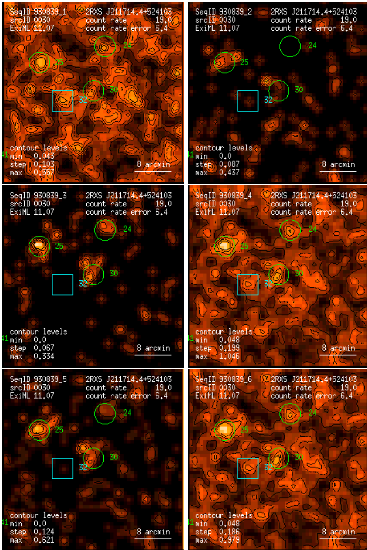
Figure 30: RASS 930839: detection 0030: band rate images, Gaussian filter: (1) PSPC channels 11 – 41, (2) 52 – 90, (3) 91 – 201, (4) 11 – 235, (5) 52 – 201, (6) 11 – 201. Broad band rates in counts/ks. Band rate contour levels in counts/ks/arcmin 2 .
