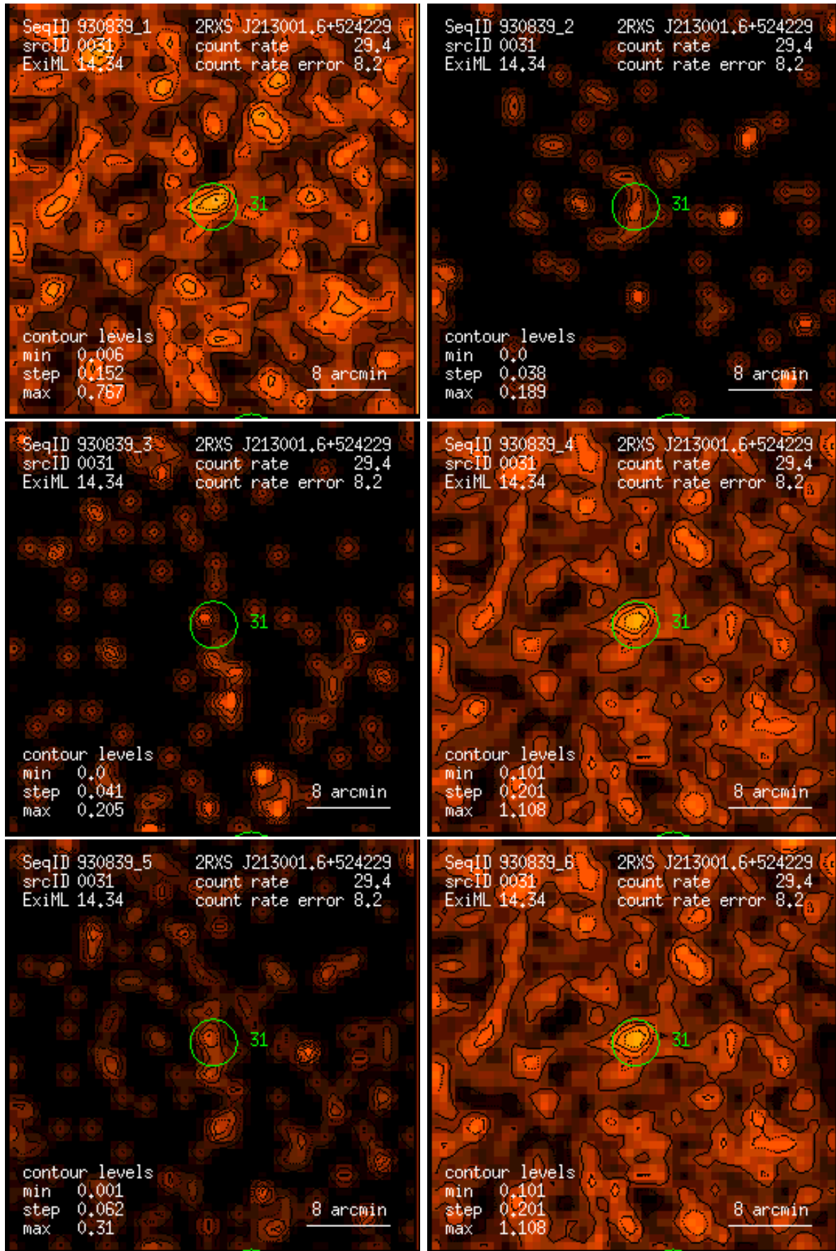
Figure 31: RASS 930839: detection 0031: band rate images, Gaussian filter: (1) PSPC channels 11 – 41, (2) 52 – 90, (3) 91 – 201, (4) 11 – 235, (5) 52 – 201, (6) 11 – 201. Broad band rates in counts/ks. Band rate contour levels in counts/ks/arcmin 2 .
