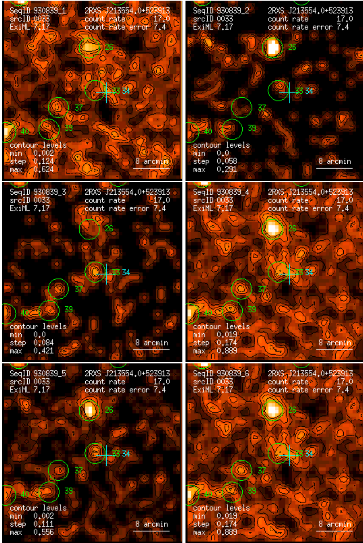
Figure 33: RASS 930839: detection 0033: band rate images, Gaussian filter: (1) PSPC channels 11 – 41, (2) 52 – 90, (3) 91 – 201, (4) 11 – 235, (5) 52 – 201, (6) 11 – 201. Broad band rates in counts/ks. Band rate contour levels in counts/ks/arcmin 2 .
