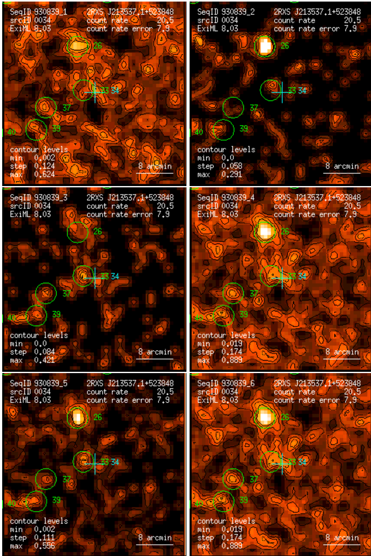
Figure 34: RASS 930839: detection 0034: band rate images, Gaussian filter: (1) PSPC channels 11 – 41, (2) 52 – 90, (3) 91 – 201, (4) 11 – 235, (5) 52 – 201, (6) 11 – 201. Broad band rates in counts/ks. Band rate contour levels in counts/ks/arcmin 2 .
