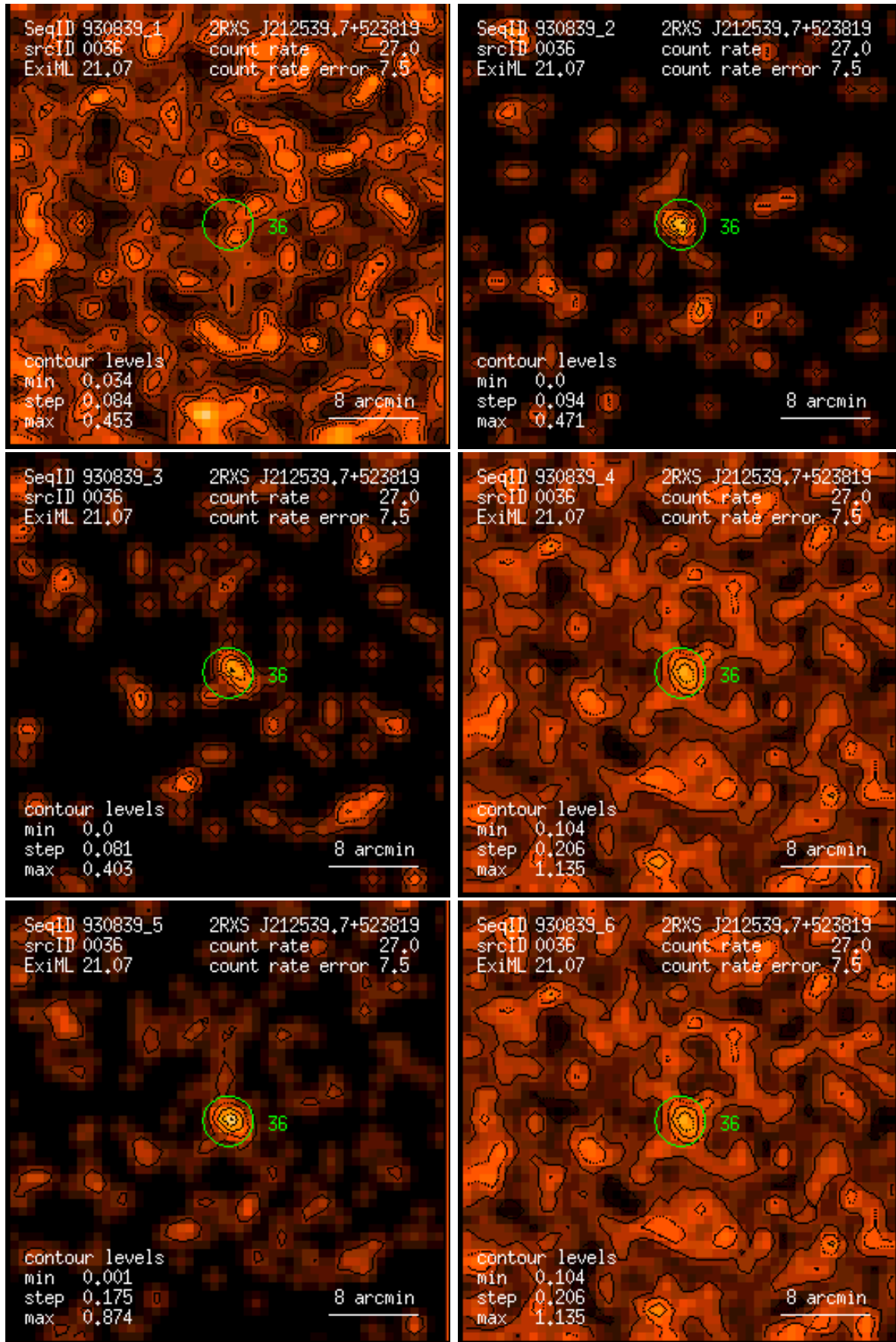
Figure 36: RASS 930839: detection 0036: band rate images, Gaussian filter: (1) PSPC channels 11 – 41, (2) 52 – 90, (3) 91 – 201, (4) 11 – 235, (5) 52 – 201, (6) 11 – 201. Broad band rates in counts/ks. Band rate contour levels in counts/ks/arcmin 2 .
