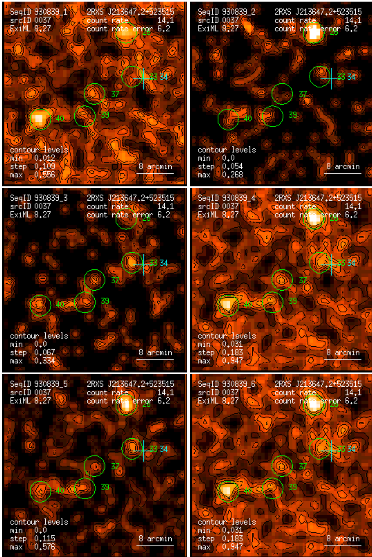
Figure 37: RASS 930839: detection 0037: band rate images, Gaussian filter: (1) PSPC channels 11 – 41, (2) 52 – 90, (3) 91 – 201, (4) 11 – 235, (5) 52 – 201, (6) 11 – 201. Broad band rates in counts/ks. Band rate contour levels in counts/ks/arcmin 2 .
