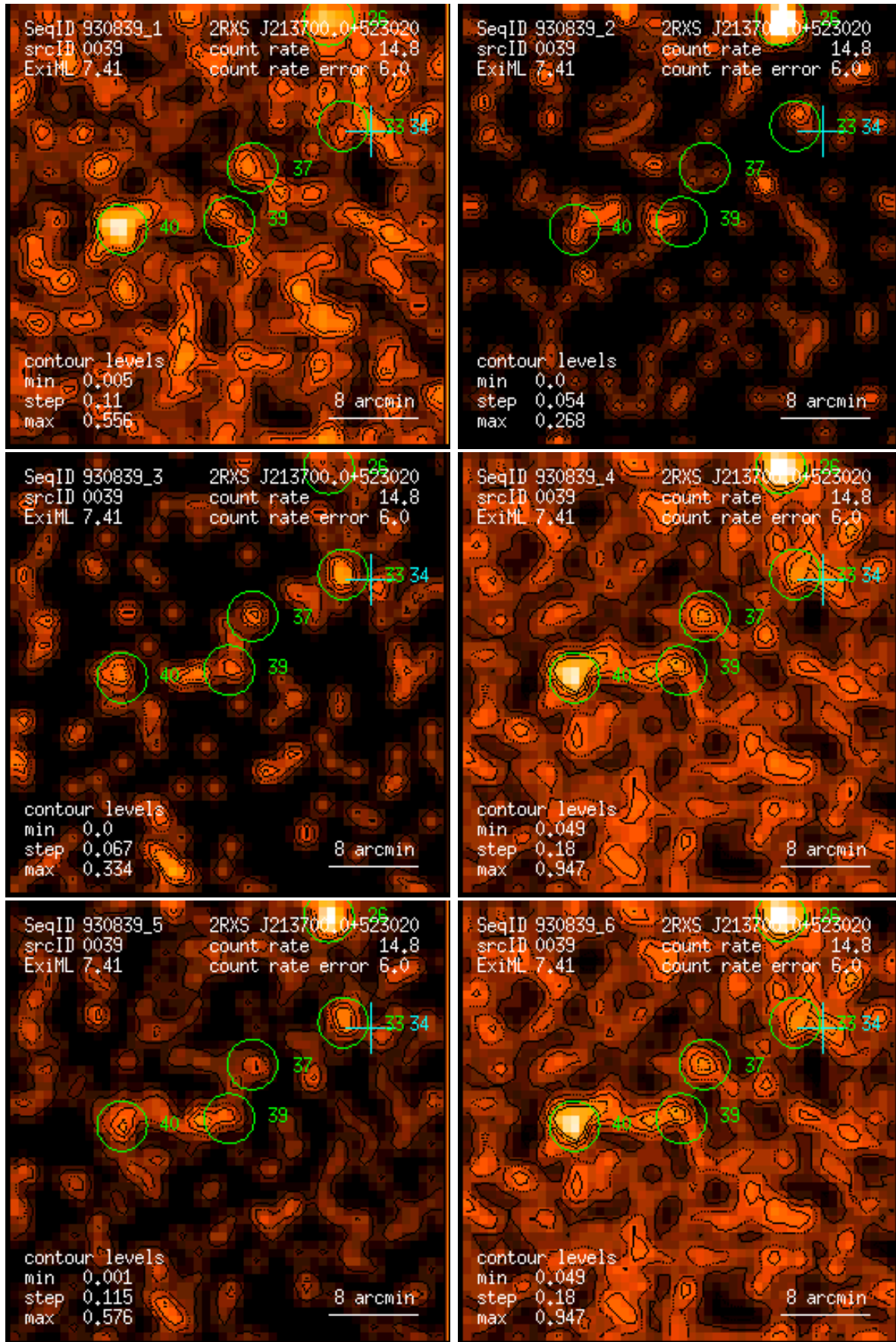
Figure 39: RASS 930839: detection 0039: band rate images, Gaussian filter: (1) PSPC channels 11 – 41, (2) 52 – 90, (3) 91 – 201, (4) 11 – 235, (5) 52 – 201, (6) 11 – 201. Broad band rates in counts/ks. Band rate contour levels in counts/ks/arcmin 2 .
