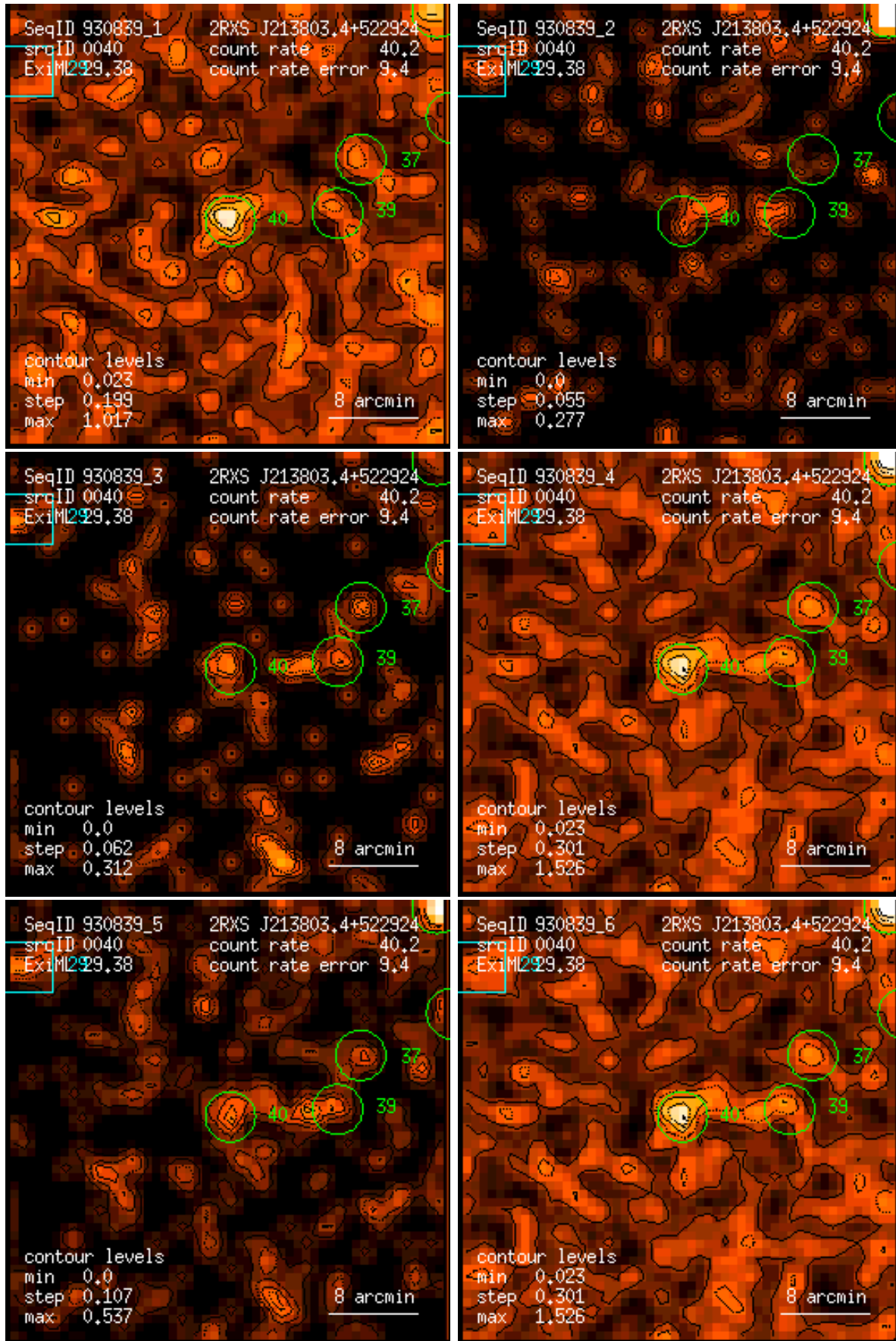
Figure 40: RASS 930839: detection 0040: band rate images, Gaussian filter: (1) PSPC channels 11 – 41, (2) 52 – 90, (3) 91 – 201, (4) 11 – 235, (5) 52 – 201, (6) 11 – 201. Broad band rates in counts/ks. Band rate contour levels in counts/ks/arcmin 2 .
