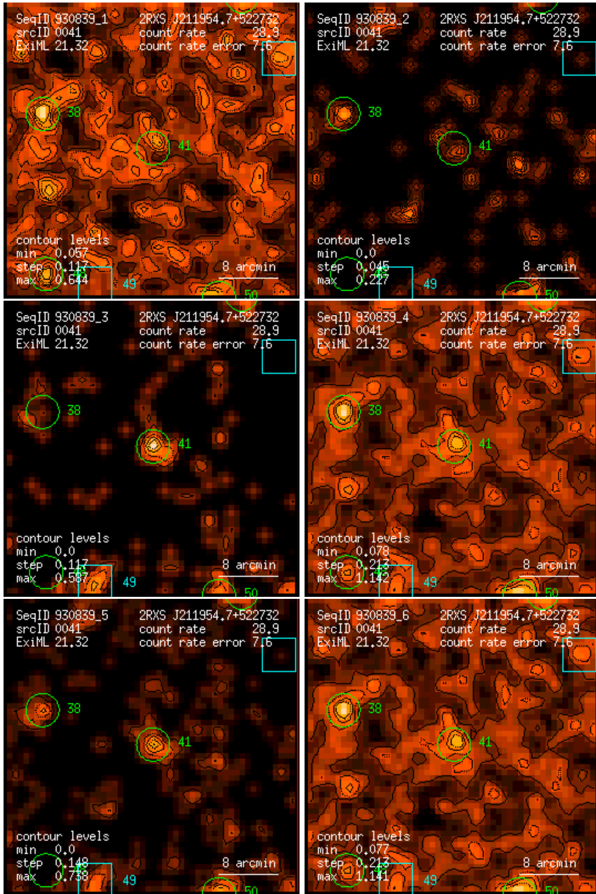
Figure 41: RASS 930839: detection 0041: band rate images, Gaussian filter: (1) PSPC channels 11 – 41, (2) 52 – 90, (3) 91 – 201, (4) 11 – 235, (5) 52 – 201, (6) 11 – 201. Broad band rates in counts/ks. Band rate contour levels in counts/ks/arcmin 2 .
