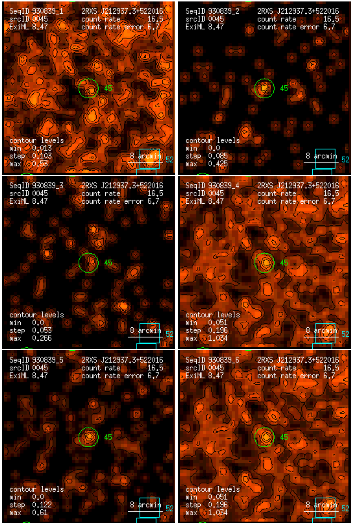
Figure 45: RASS 930839: detection 0045: band rate images, Gaussian filter: (1) PSPC channels 11 – 41, (2) 52 – 90, (3) 91 – 201, (4) 11 – 235, (5) 52 – 201, (6) 11 – 201. Broad band rates in counts/ks. Band rate contour levels in counts/ks/arcmin 2 .
