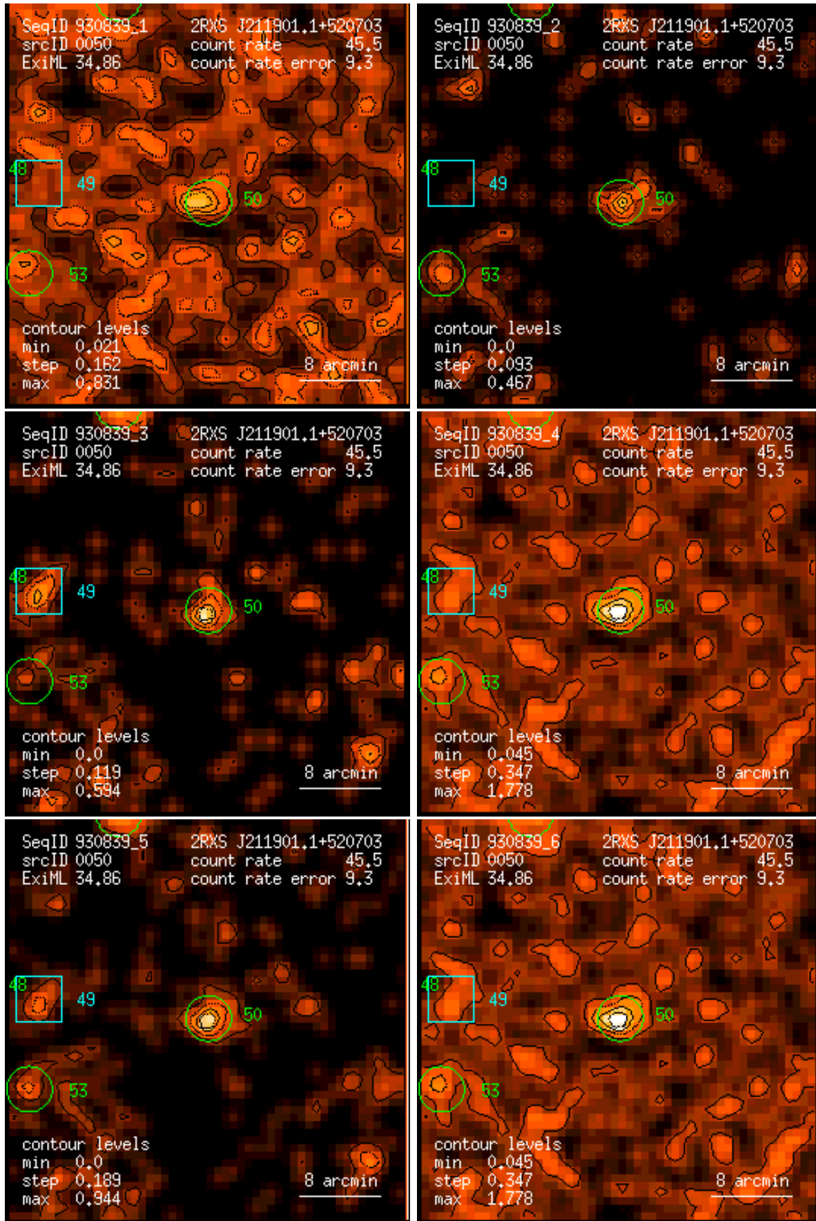
Figure 50: RASS 930839: detection 0050: band rate images, Gaussian filter: (1) PSPC channels 11 – 41, (2) 52 – 90, (3) 91 – 201, (4) 11 – 235, (5) 52 – 201, (6) 11 – 201. Broad band rates in counts/ks. Band rate contour levels in counts/ks/arcmin 2 .
